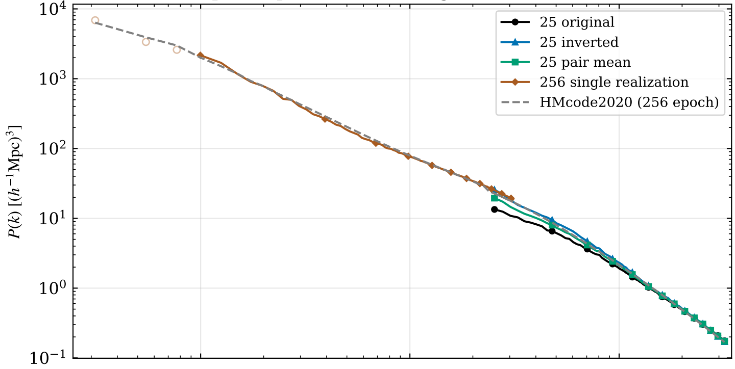
PL: 25 phase pair and 256 single realization, z \sim 1.07
