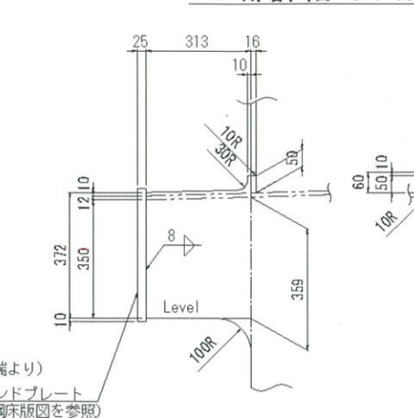
"A"部詳細 S=1:10
