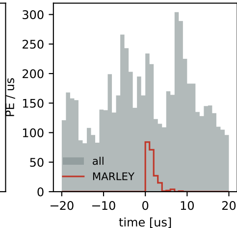
zoom: \pm 20 us around the neutrino
