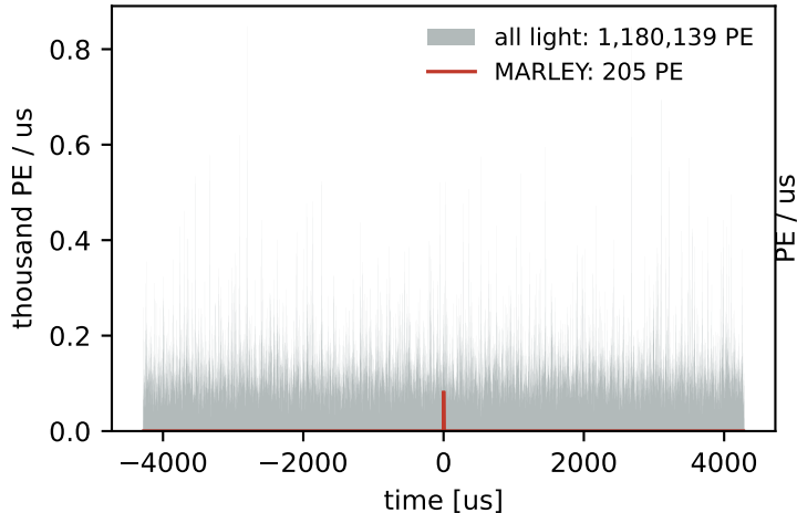
mixed event 0: the whole light readout window
