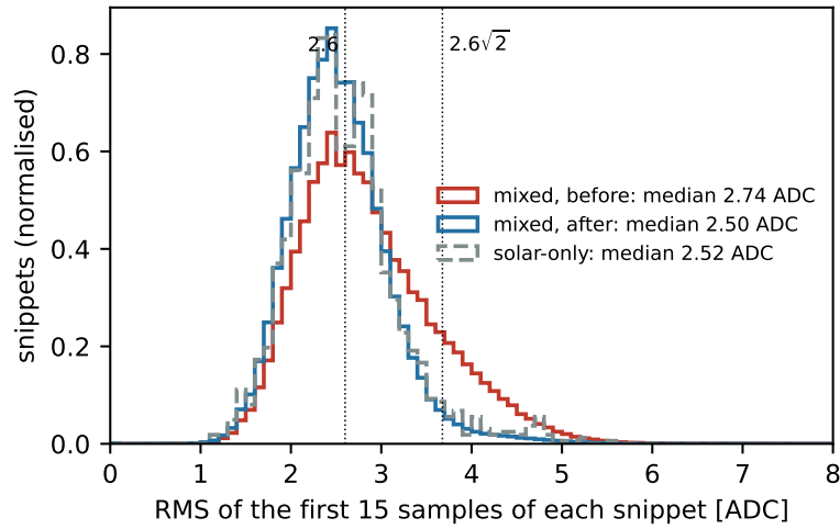
Figure 4: Bug B, all events. Top: fraction of samples stored twice, of duplicate OpHits (same channel and peak time) and of the OpHit PE they carry, before and after the fix. The 0.07 % of samples still stored twice after the fix are the 20-sample pre-trigger of a new snippet re-reading the end of the previous one, which is how the readout is modelled. Bottom: baseline noise of the snippets; the noise is added twice where ranges overlap (expected RMS 2.6\sqrt{2} = 3.7 ADC).
