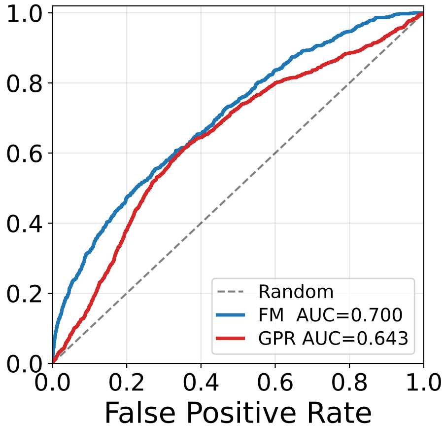
K one-vs-rest
