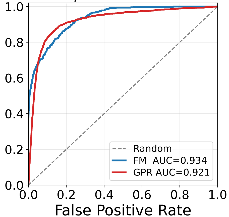
p one-vs-rest
