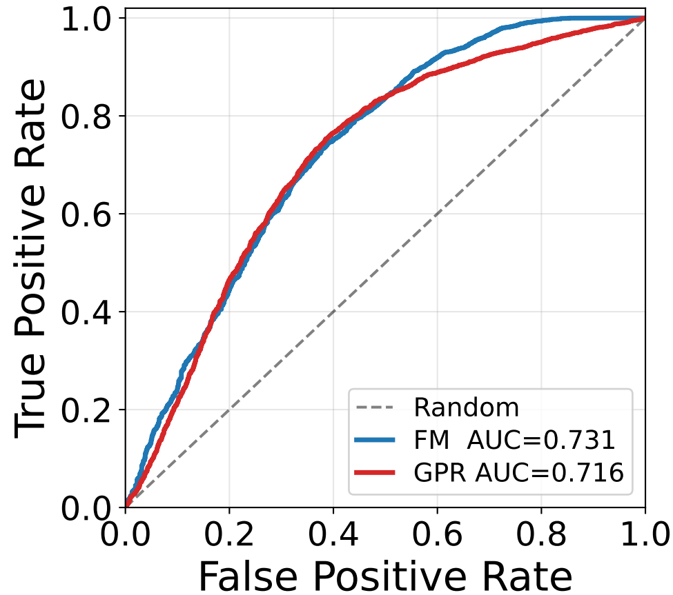
\pi one-vs-rest
