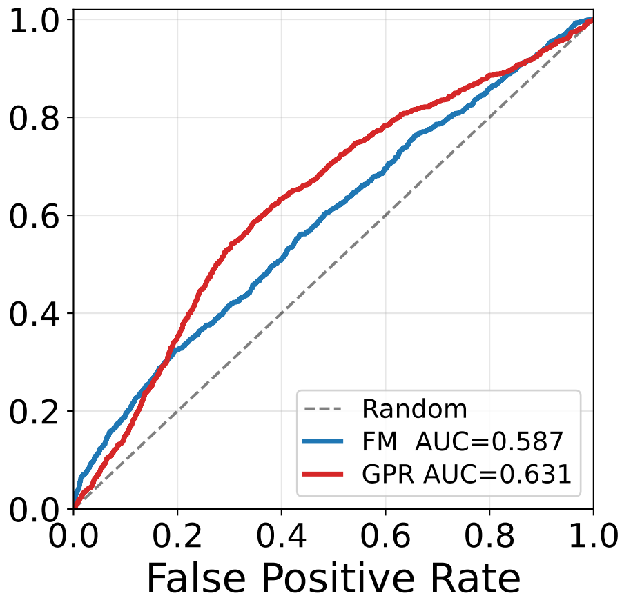
K one-vs-rest
