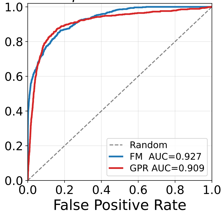
p one-vs-rest
