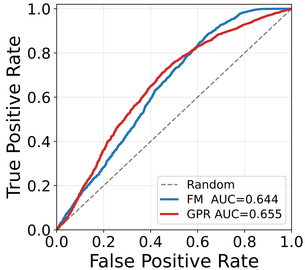
\pi one-vs-rest
