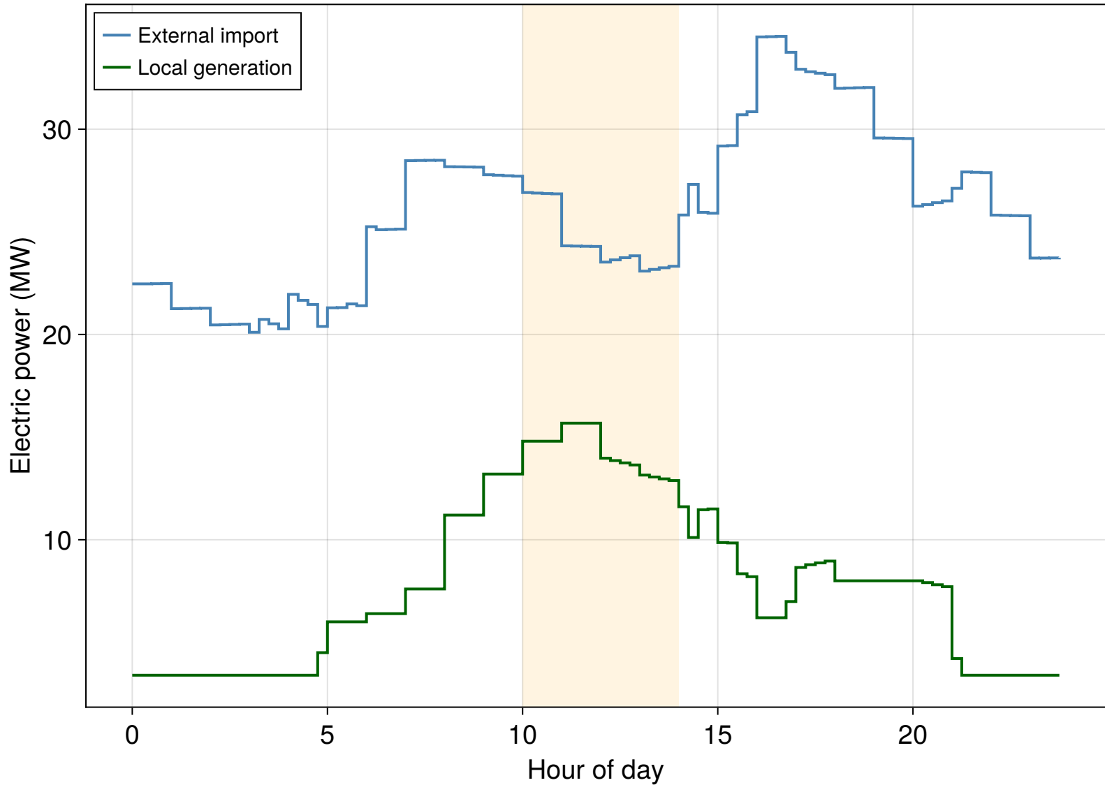
Economic normal schedule; event inherits this state
