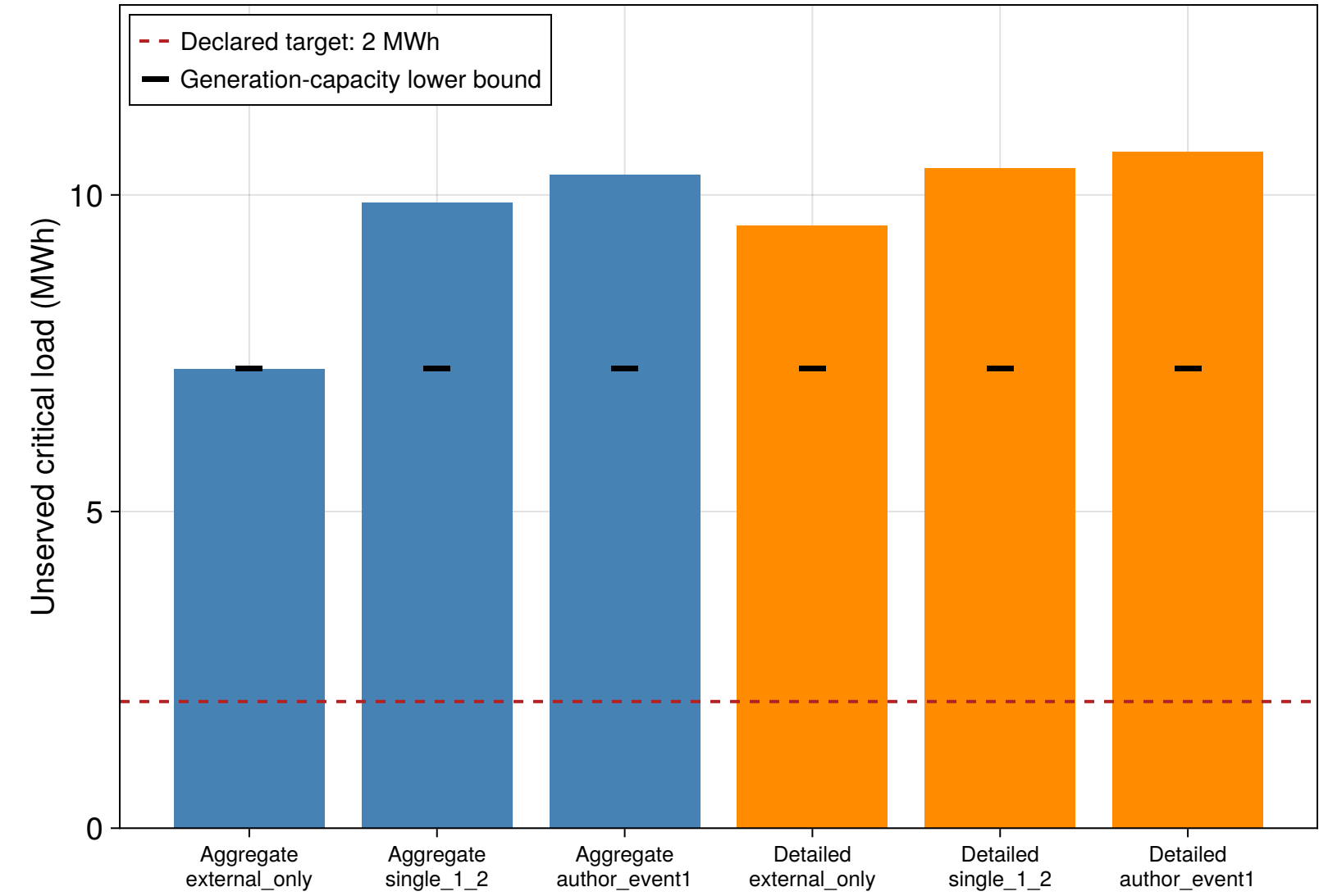
Four-hour critical electricity not supplied
