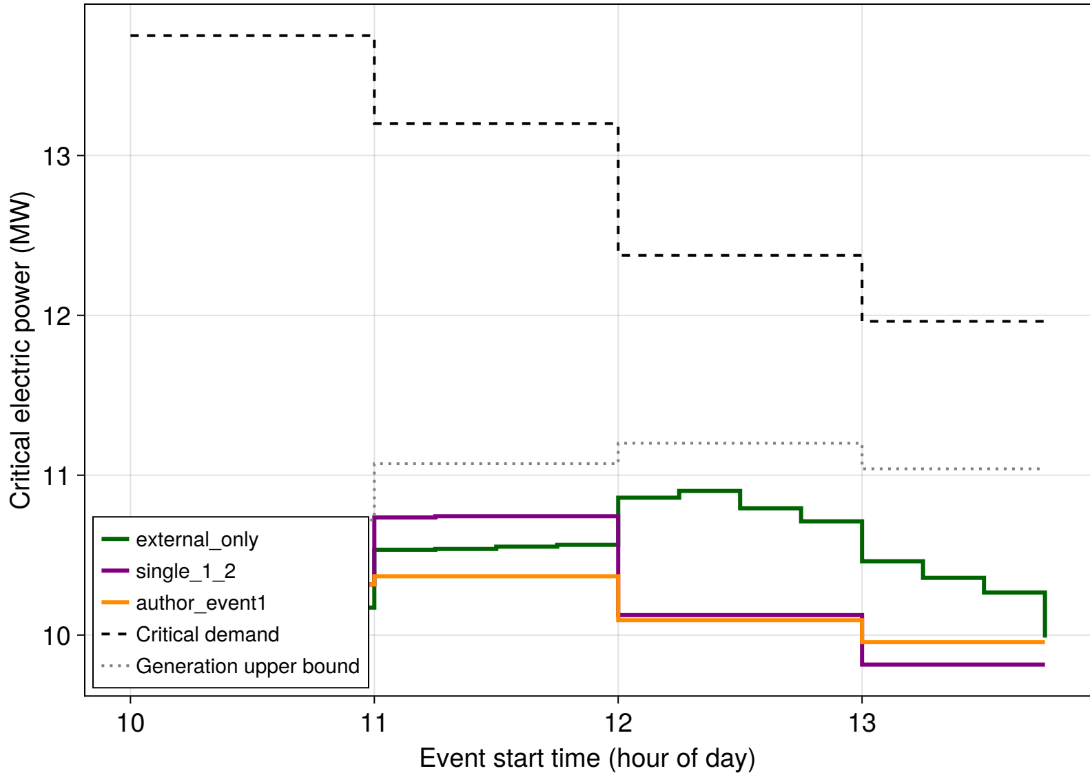
Detailed fixed-flow restoration
