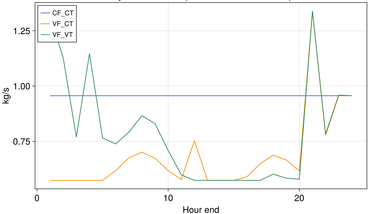
Pipe 1 mass flow (saved direct candidates)
