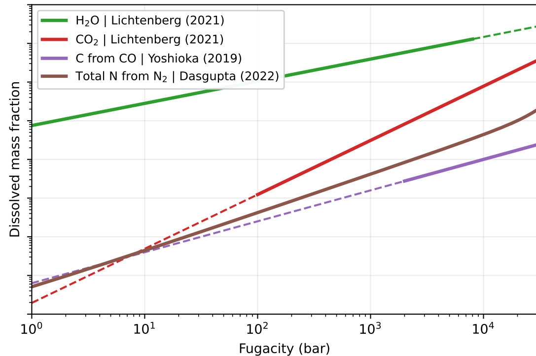
Mass-fraction laws
