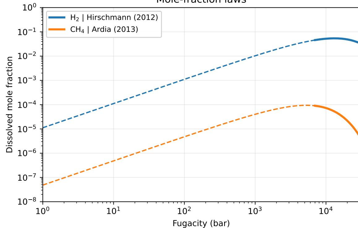
Mole-fraction laws
