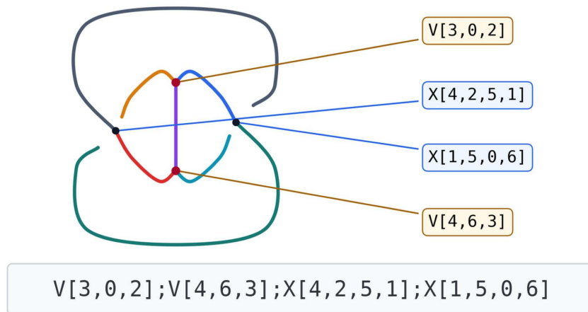
(b) Projection / PD-Code Analysis
