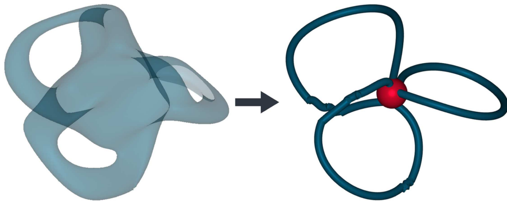
(a) Knotted/Spatial Graph Construction
