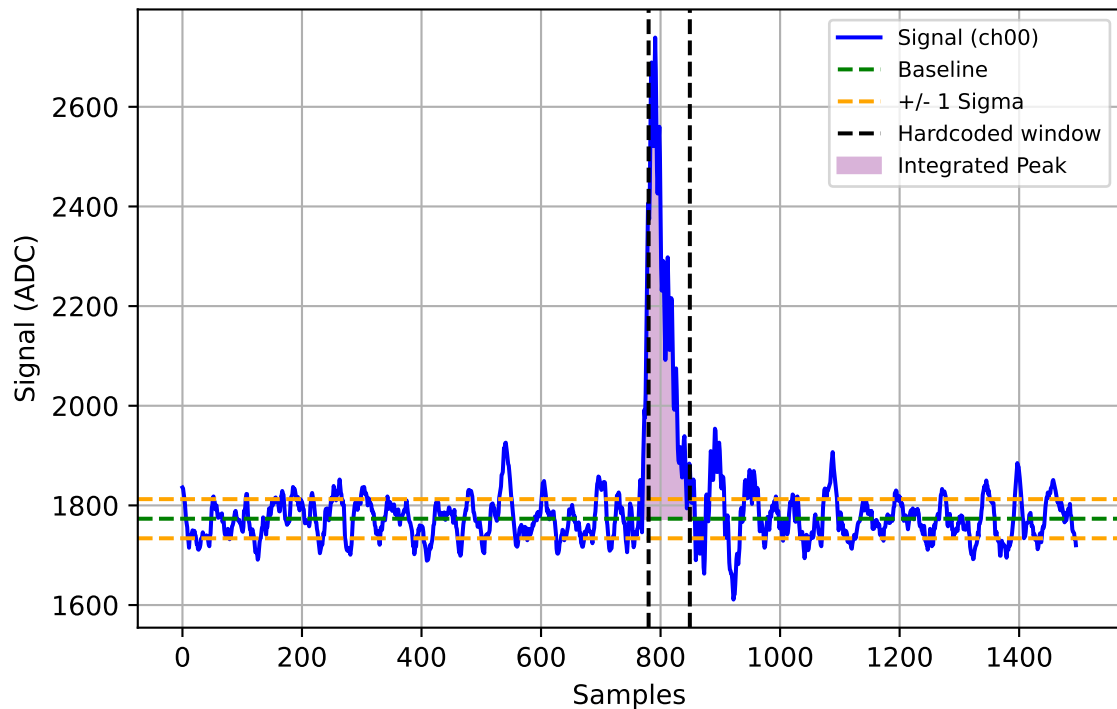
Sample Signal 1 (Row: 78513, Ch: ch00) 90.0 °C / 363.1 K LED: 2.5 V | SiPM: 56.0 V
