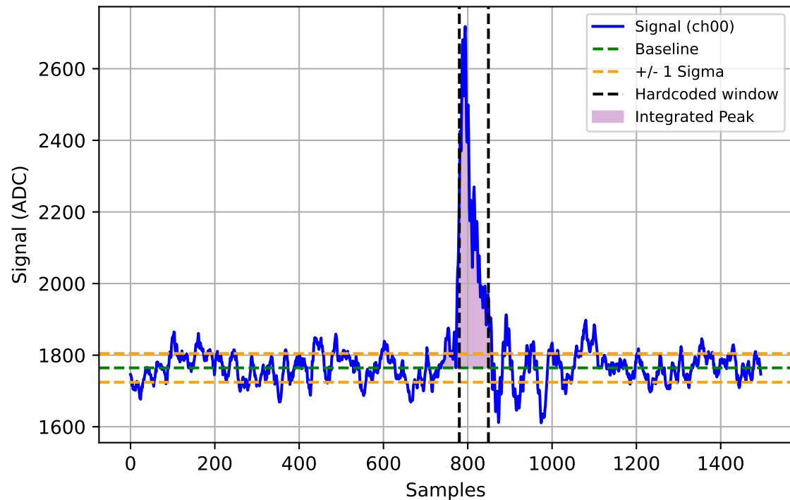
Sample Signal 2 (Row: 31499, Ch: ch00) 90.0 °C / 363.1 K LED: 2.5 V | SiPM: 56.0 V
