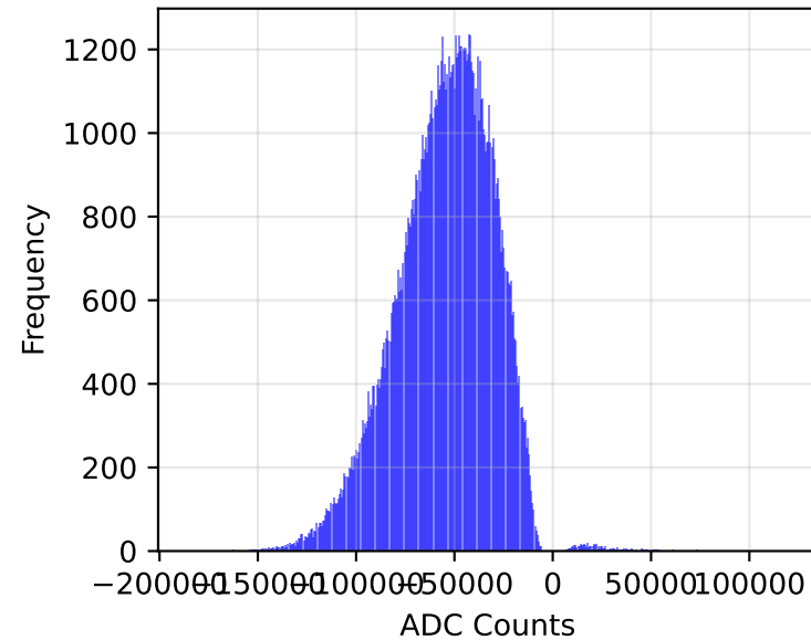
ch03 (REJECTED: \chi^2/\text{NDF} > 2 )
