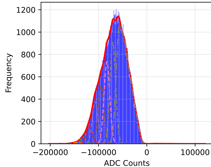
ch10, with \chi^2/\text{NDF} = 0.737
