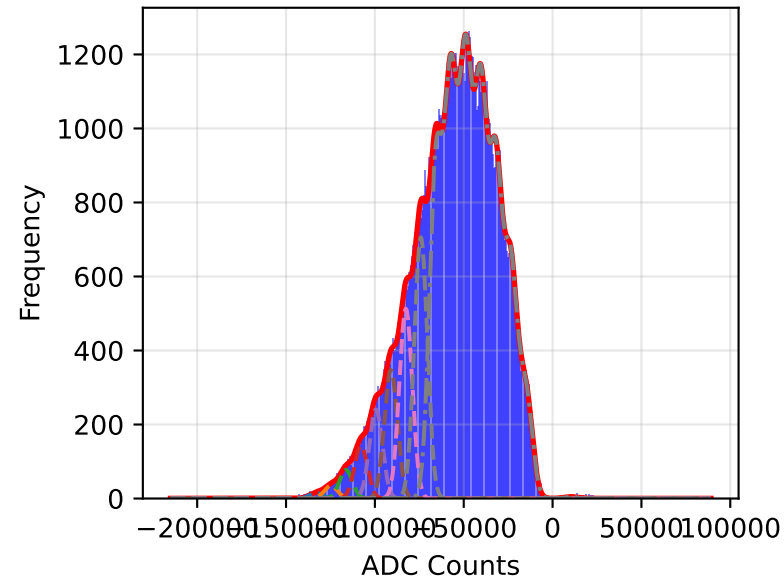
ch11, with \chi^2/\text{NDF} = 1.212
