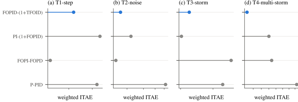
Figure 4: Weighted ITAE in the four test cases, best robust tuning of each structure (logarithmic axes).
