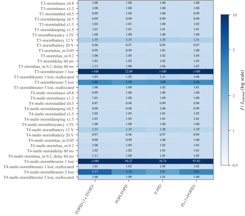
Figure 6: Cost of each variant relative to the nominal test case, per structure, best robust tuning (the controllers are not retuned).
