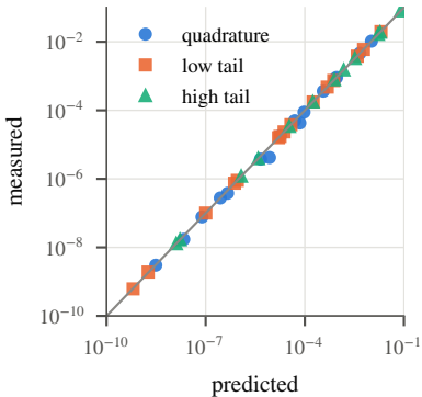
(a) discrete time (GL weights)
