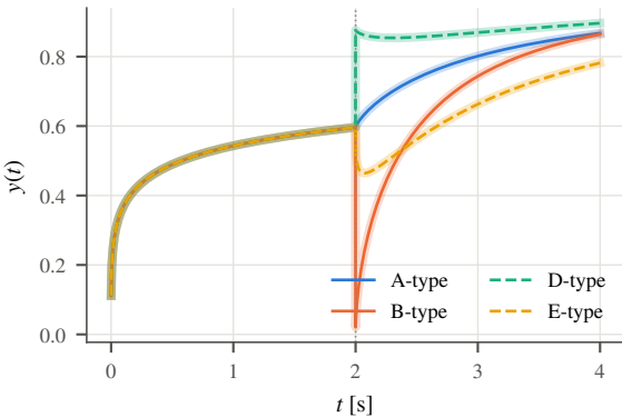
(a) {}^T D^{\alpha(t)} y + y = 1 , \alpha: 0.3 \rightarrow 0.8 at 2 s
