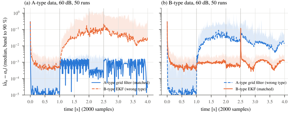
Fig. 6 Order tracking at 60 dB: absolute error of the order estimate (median over 50 runs, band to the 90th percentile). Solid: filter of the type that generated the data; dashed: filter of the other type. Dotted lines mark the start and end of the ramp and the jump
