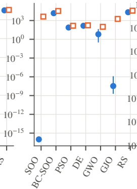
(c) rosenbrock
