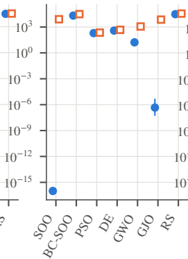
(b) rastrigin
