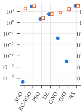
(a) sphere
