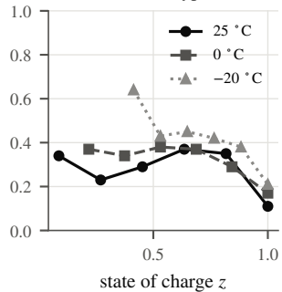
(c) order law, B-type
