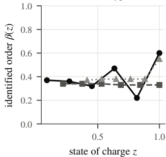
(b) order law, A-type
