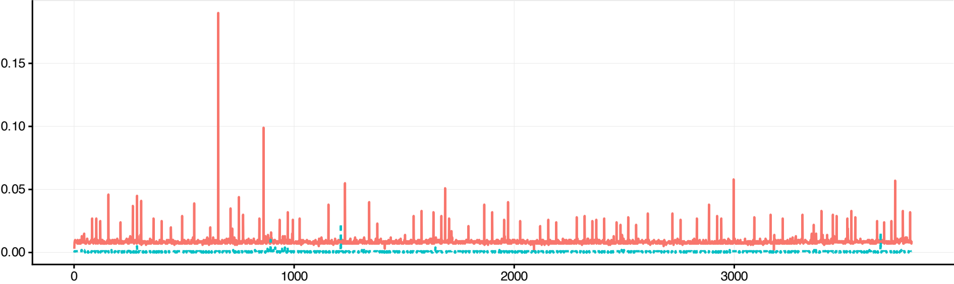
Window index
