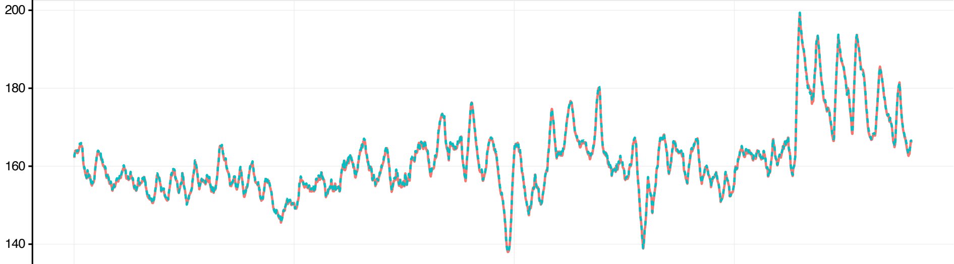
Per-window runtime
