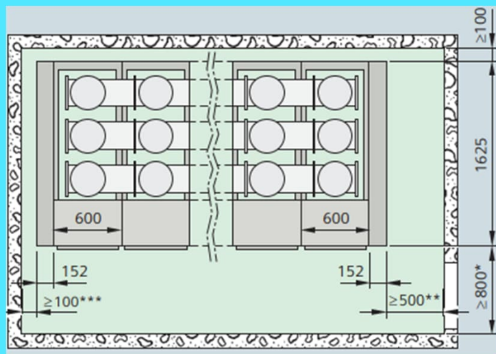
靠墙布置
