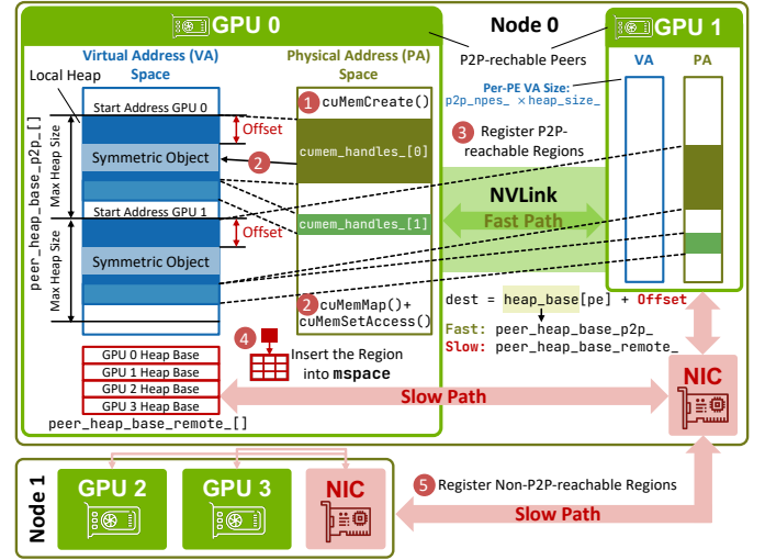
Fig. 1. Virtual-memory-based symmetric-heap setup in NVSHMEM for two nodes, each with two GPUs and one NIC. The numbered markers 1–5 show the main steps taken when new physical memory is allocated.
