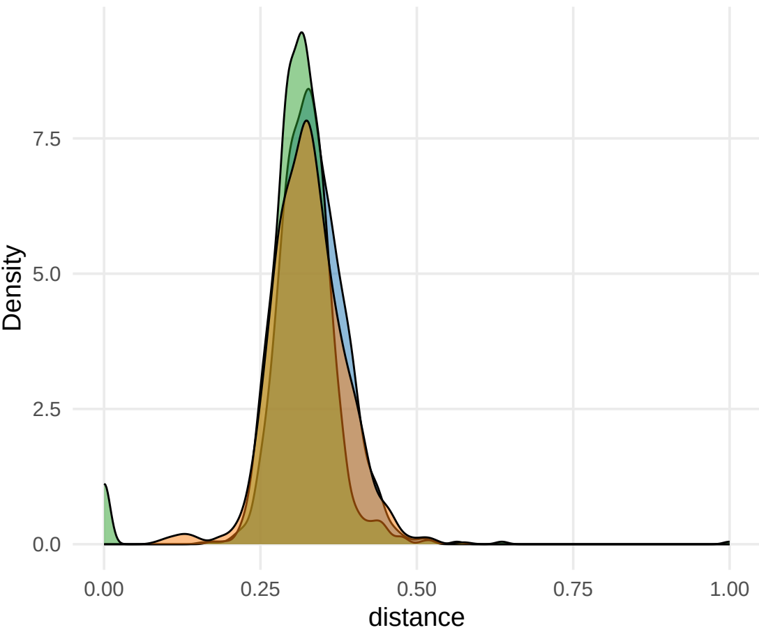
distance Distribution
