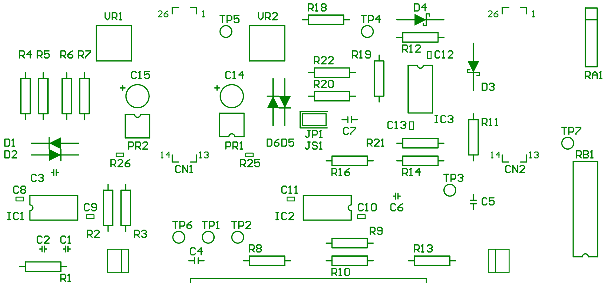
Coin Selector Circuit Board
