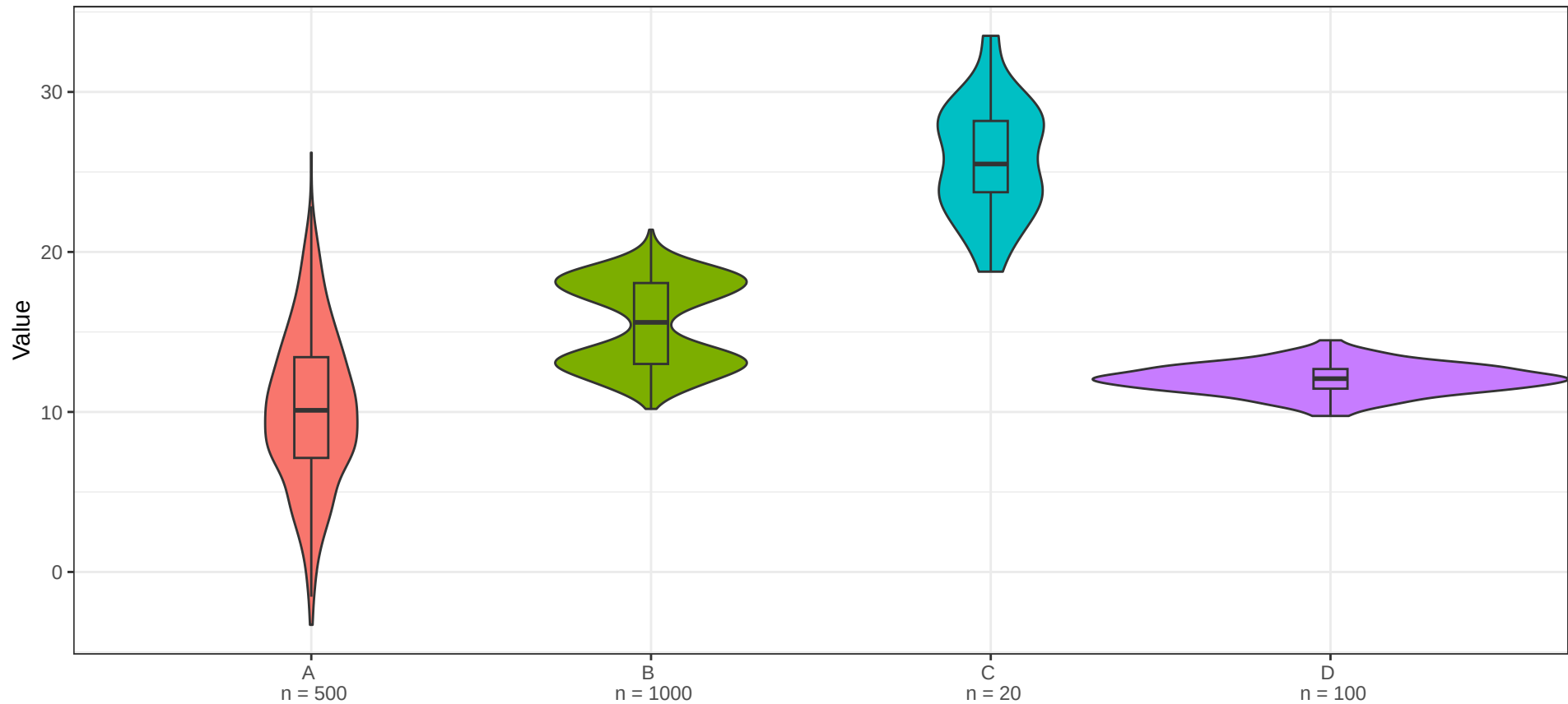
Boxplot + Violin
