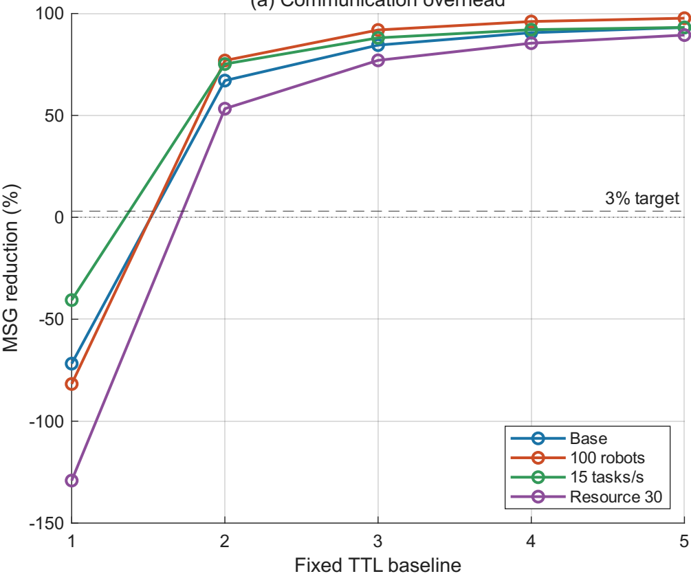
(a) Communication overhead
