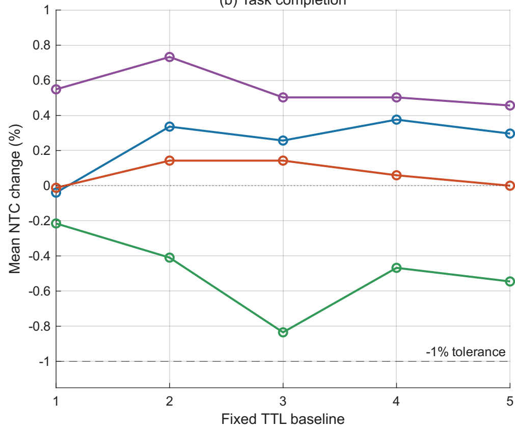
(b) Task completion
