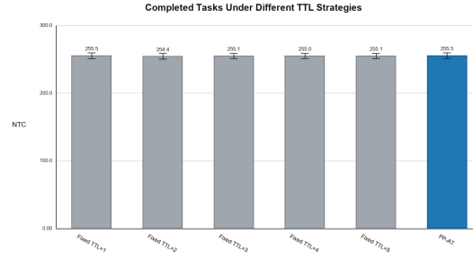
Figure 3. NTC comparison under MPDM (mean ± sample standard deviation).
