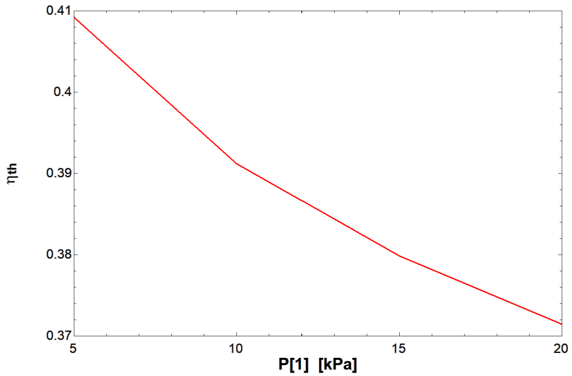
Figure 10: Parametric, efficiency (thermal) as affected by condenser pressure)
