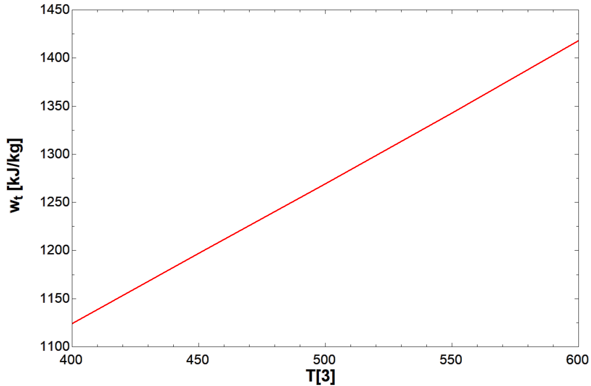
Figure 13: Parametric, work done by turbine (work out w/ units) as affected by boiler temperature (5 intervals of temp displayed on x-axis)
