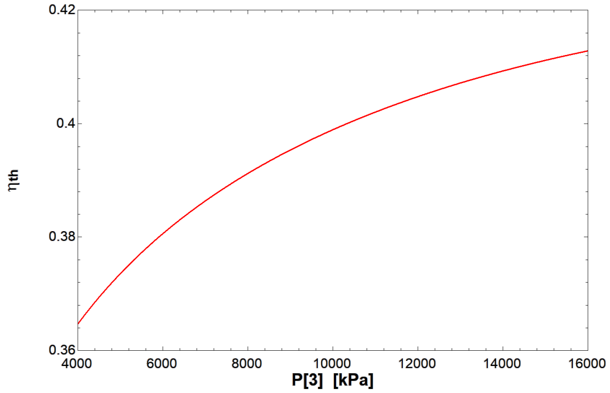
Figure 11: Parametric, Thermal efficiency as affected by boiler pressure
