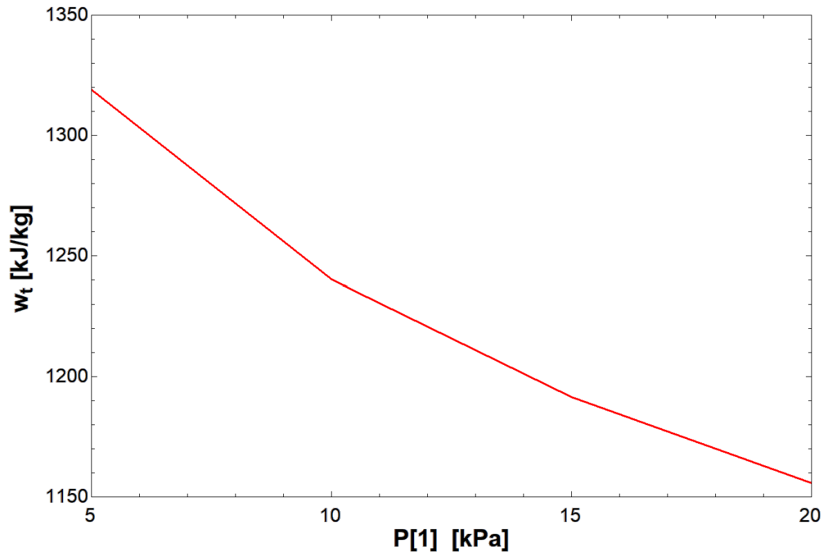
Figure 9: Parametric, Condenser Pressure x axis work done by turbine y axis. parametric graph, 4 intervals of pressure displayed on x axis
