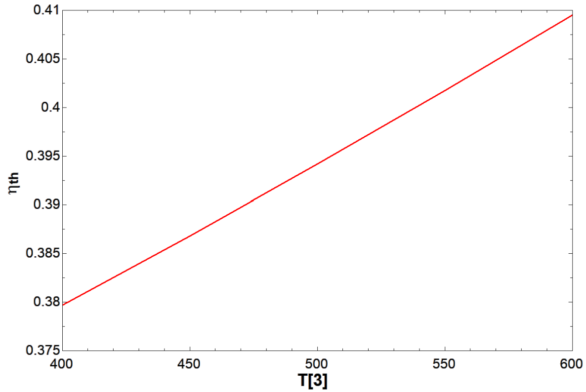
Figure 12: Parametric, thermal efficiency as affected by temperature at boiler exit
