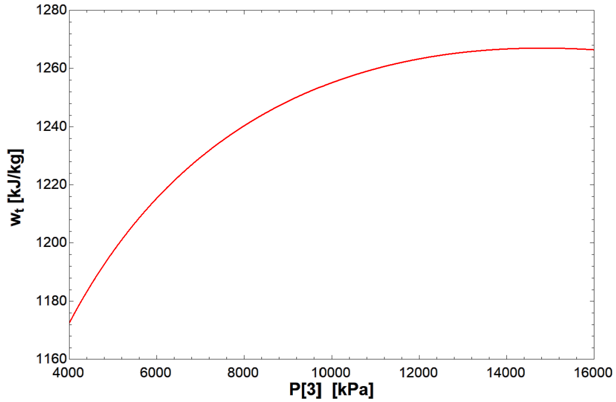
Figure 8: Parametric, work done by the turbine work output as affected by variable pressure exiting the boiler.
