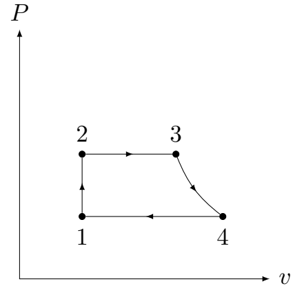
Figure 3: Ideal Rankine Cycle P-v Diagram
