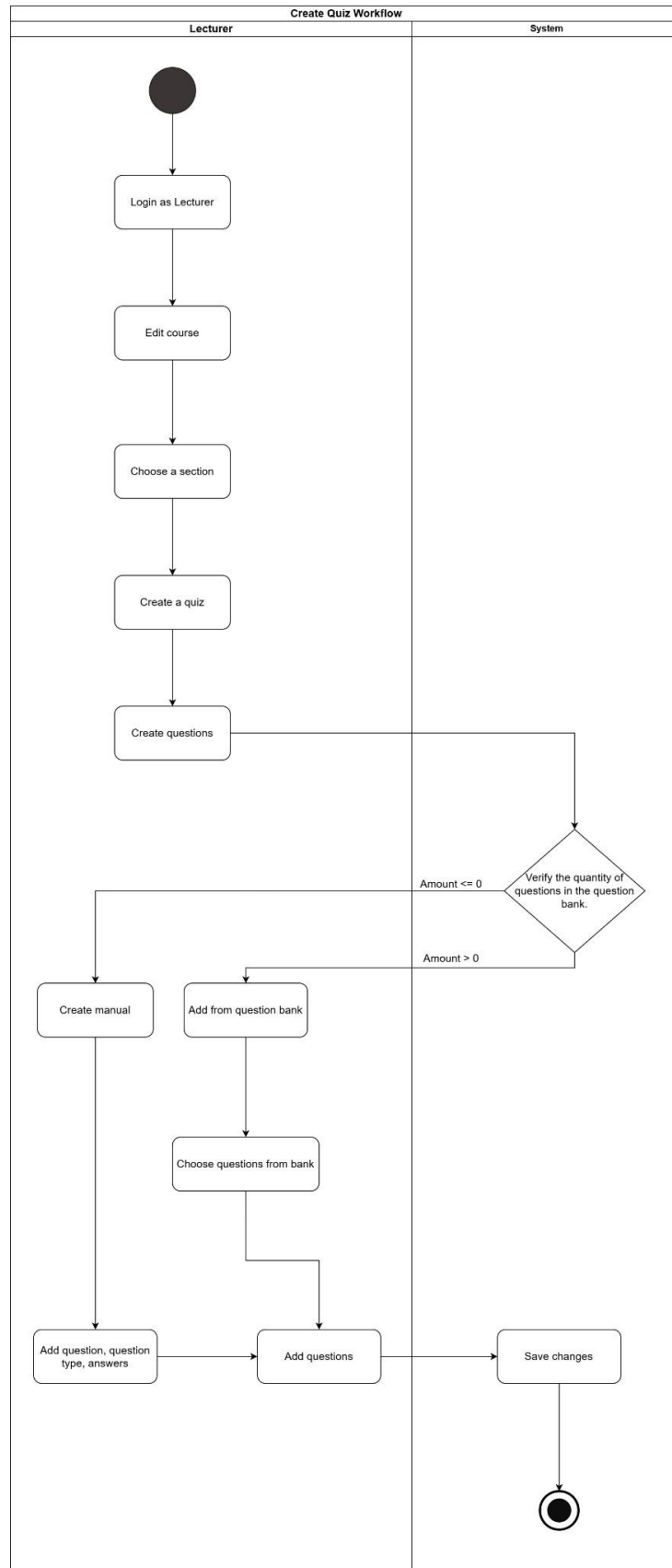
Figure 1.2.4 - Main workflow create quiz
