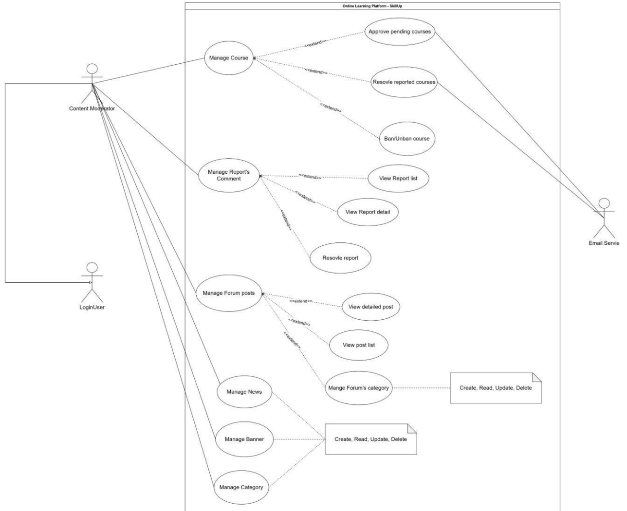
Figure 1.3.3.5 - use case content moderator diagram
