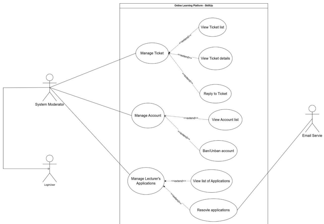
Figure 1.3.3.6 - use case system moderator diagram
