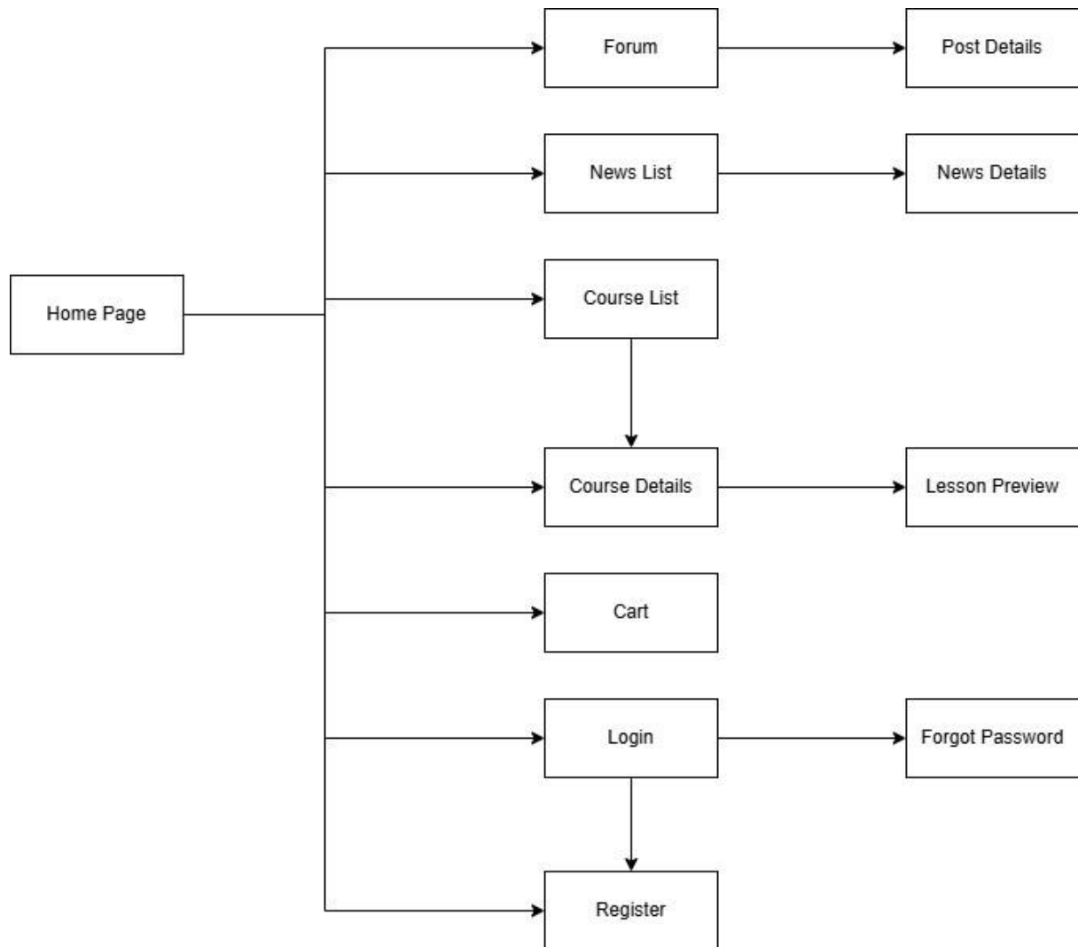
Figure 1.4.1.1 - Guest Screens Flo
