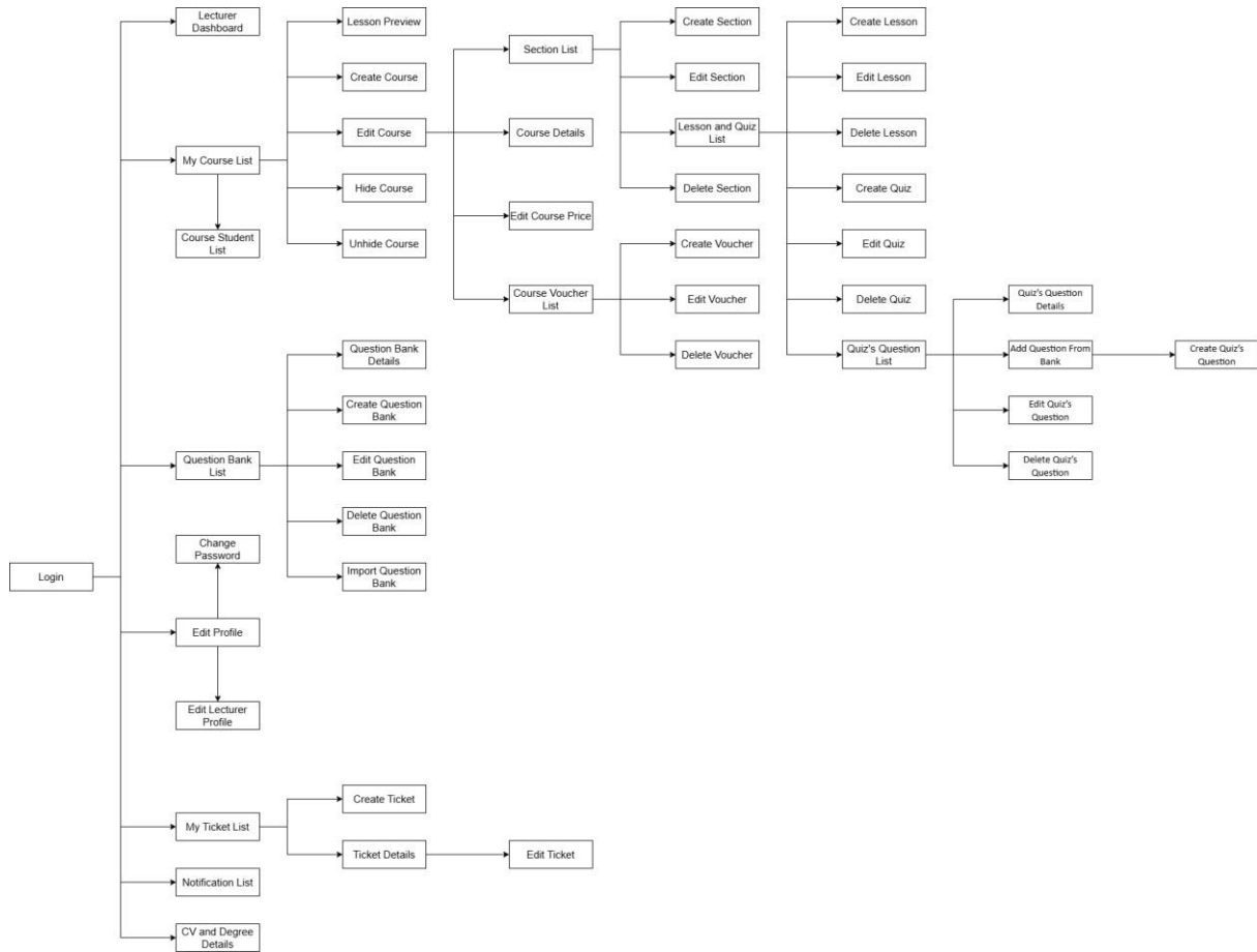
Figure 1.4.1.3 - Lecturer Screens Flow 1.4.1.4
