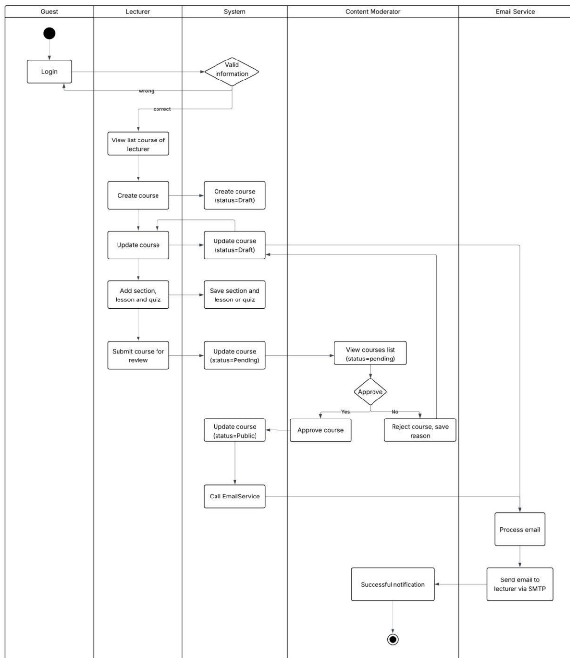
Figure 1.2.2 - Main workflow create course
