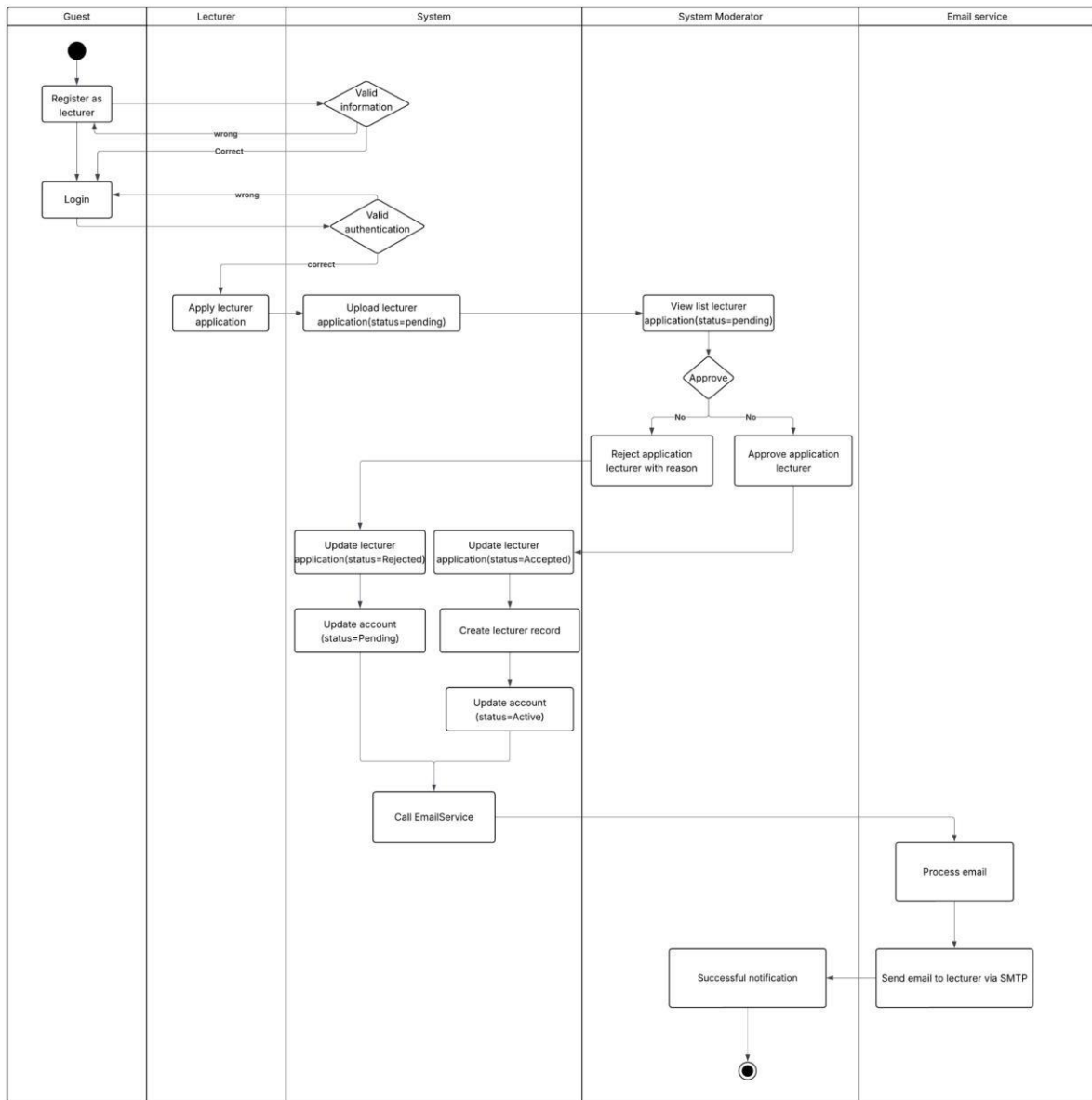
Figure 1.2.1 - Main workflow register to become a lecturer
