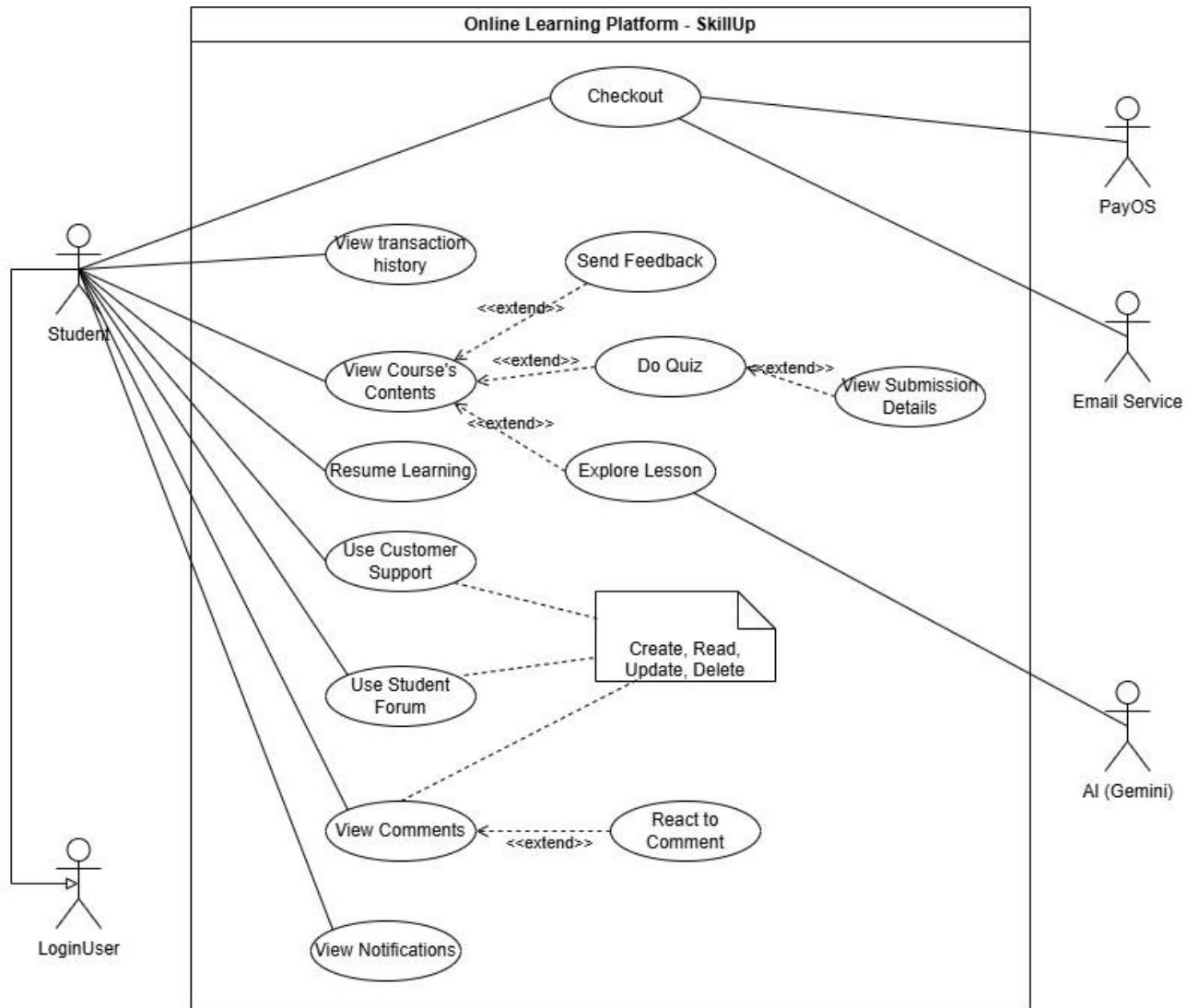
Figure 1.3.3.3 - use case student diagram
