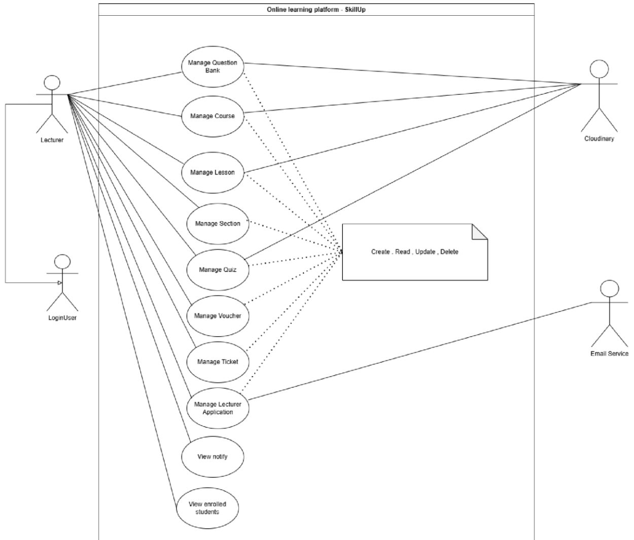
Figure 1.3.3.4 - use case lecturer diagram
