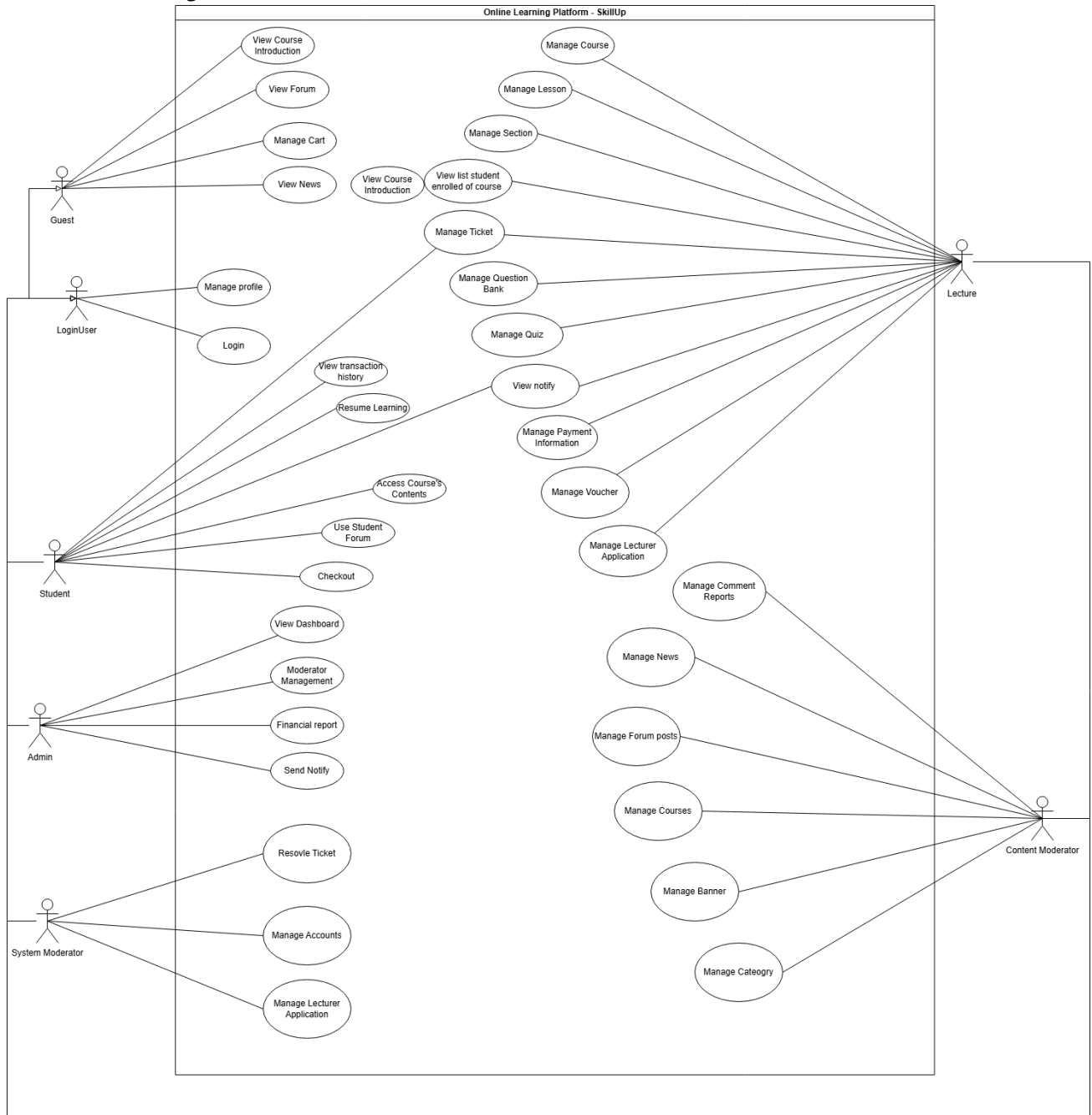
Figure 1.3.3 - Overview use case diagram
