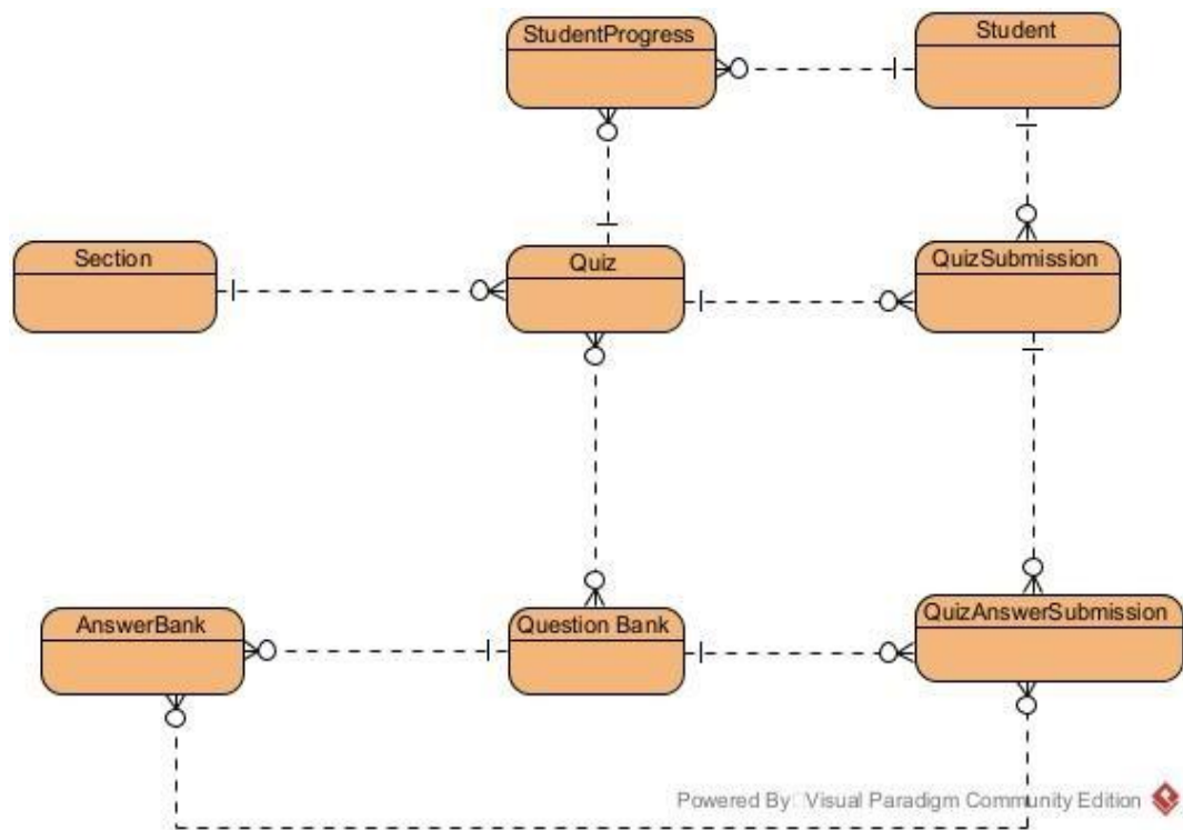
Figure 1.5.2 - Quiz entity relationship diagram
