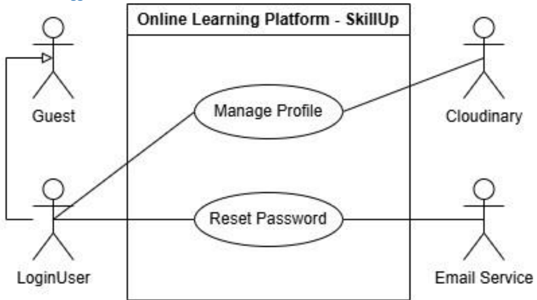
Figure 1.3.3.1 - use case logged in user diagram
