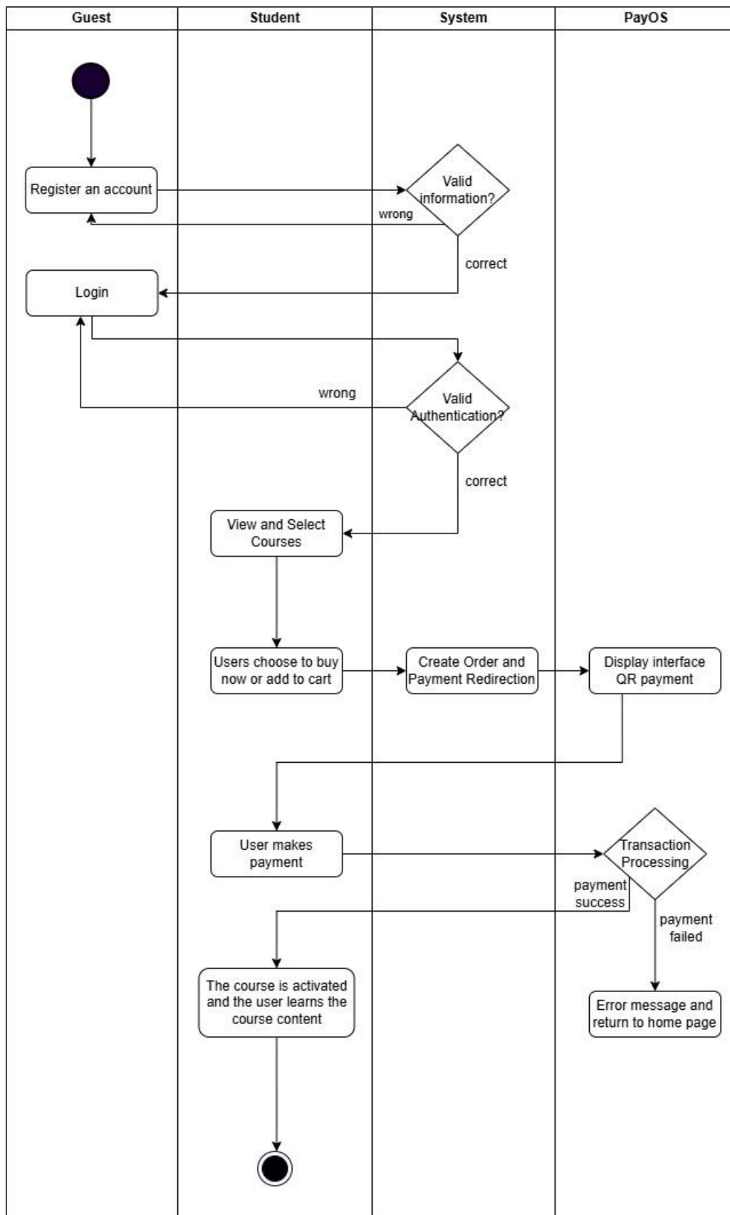
Figure 1.2.3 - Main workflow buy course and learning materials
