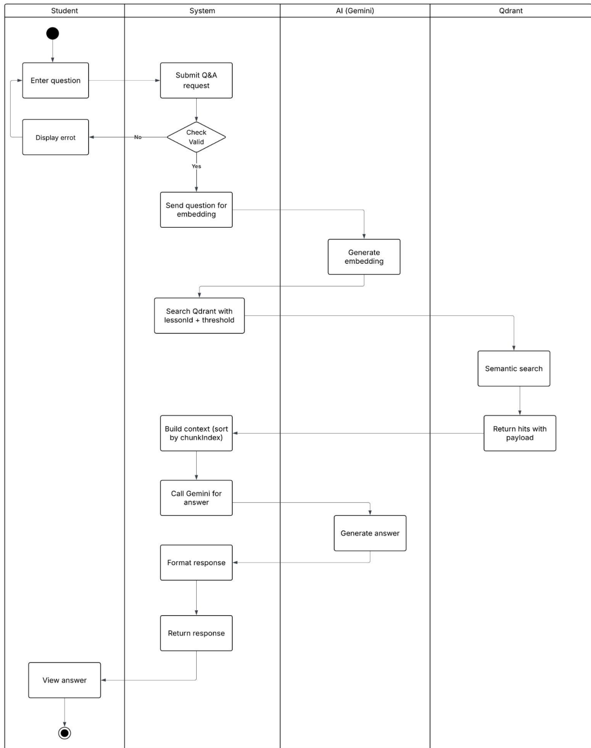
Figure 1.2.5 - Main workflow AI lesson Q&A
