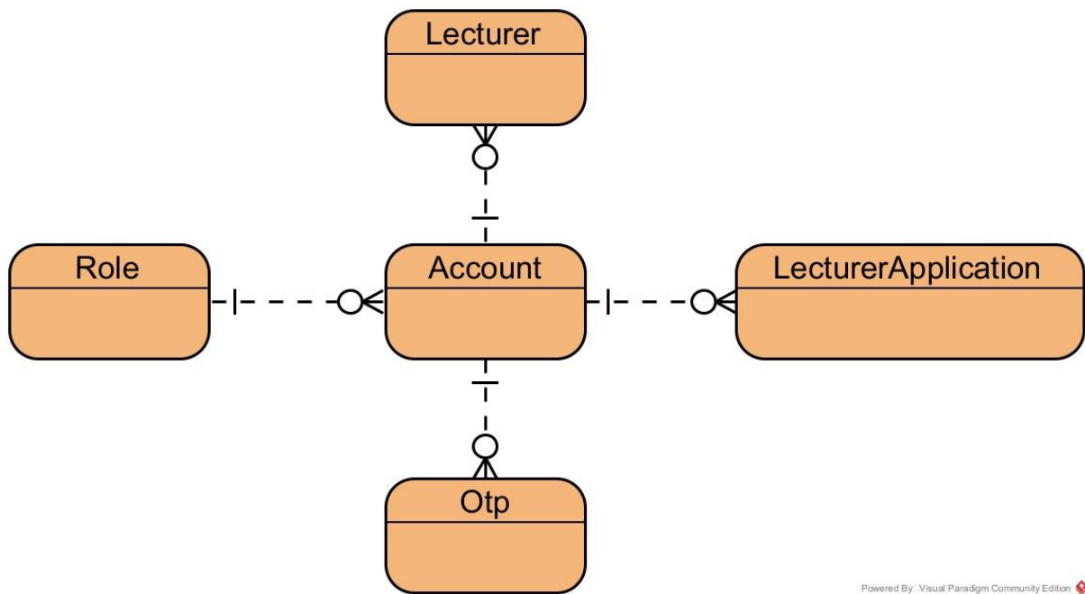
Figure 1.5.4 - LecturerApplication relationship diagram
