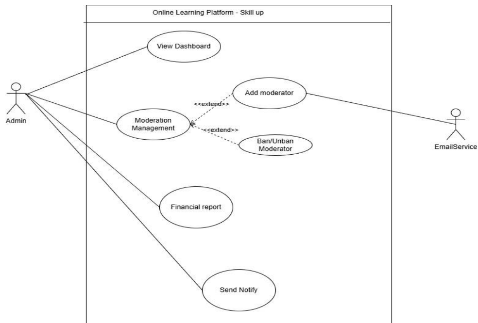
Figure 1.3.3.7 - use case admin diagram
