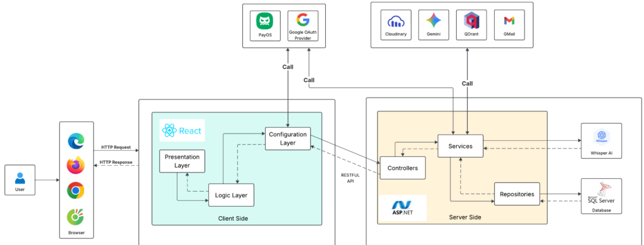
Figure 1.1 SkillUp System Architecture
