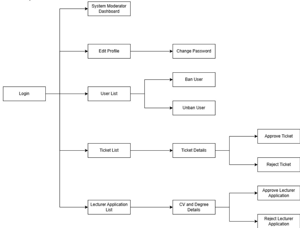
Figure 1.3.1.5 - System moderator Screens Flow
