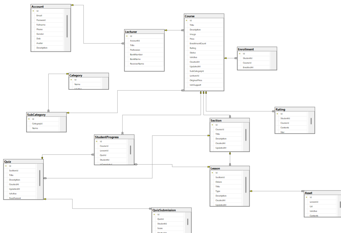
Figure 2.4. - data tables related to course
