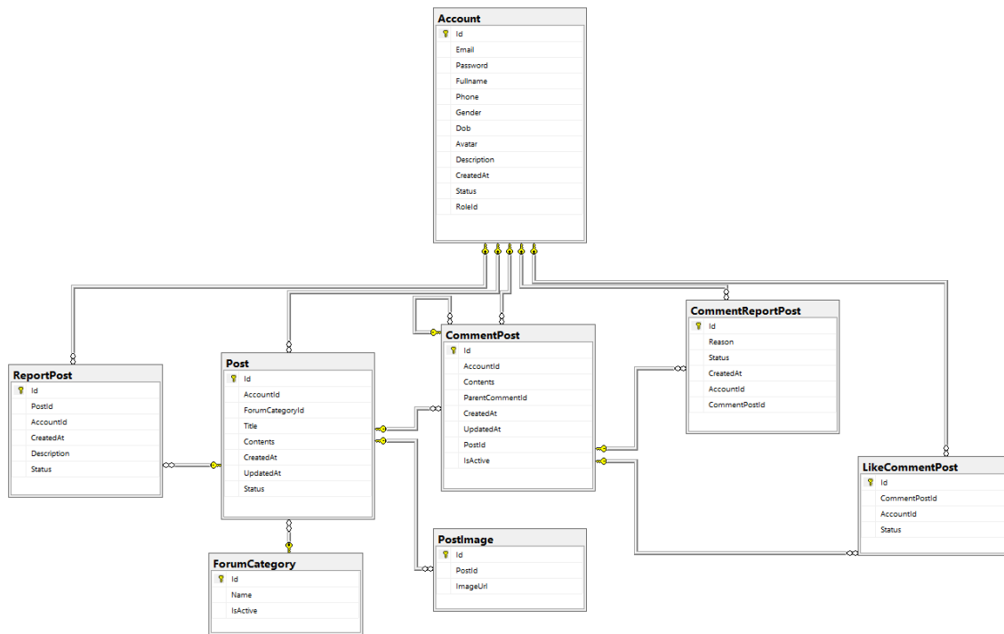
Figure 2.3. - data tables related to forum
