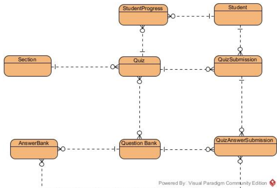
Figure 1.5.2 - Quiz entity relationship diagram
