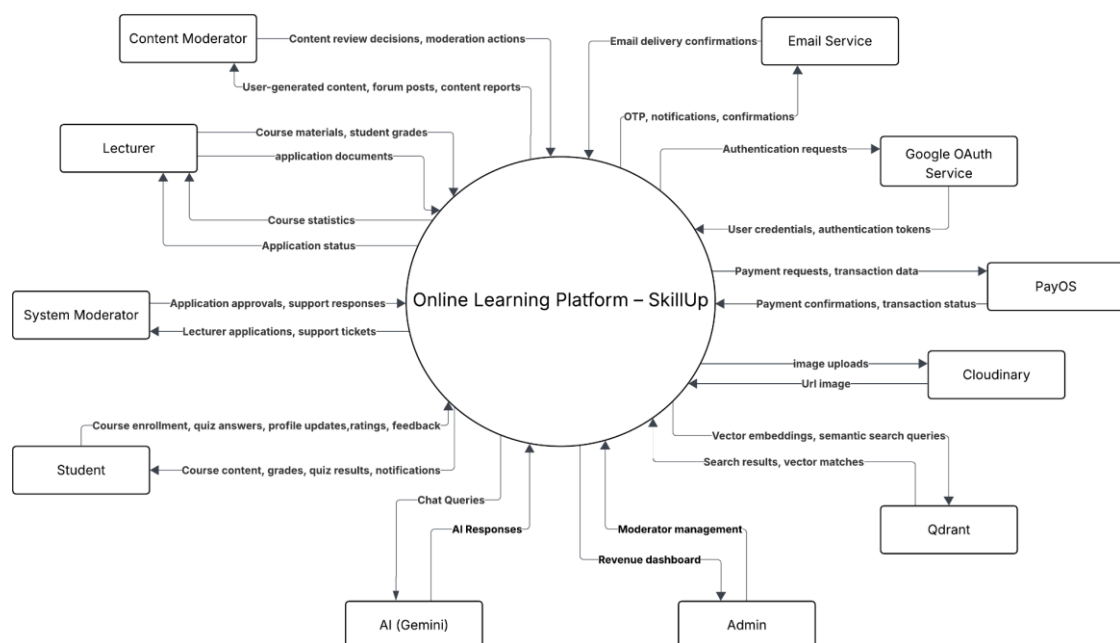
Figure 1.1: Context Diagram
