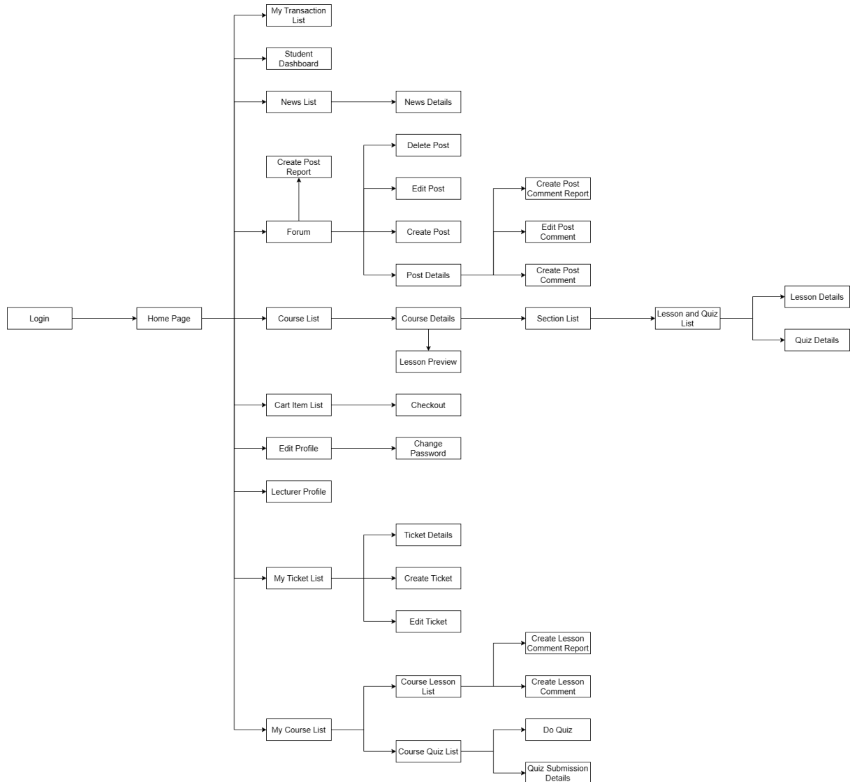
Figure 1.3.1.6 - Student Screens Flow
