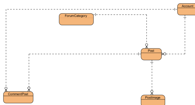
Figure 1.5.5 - Forum relationship diagram
