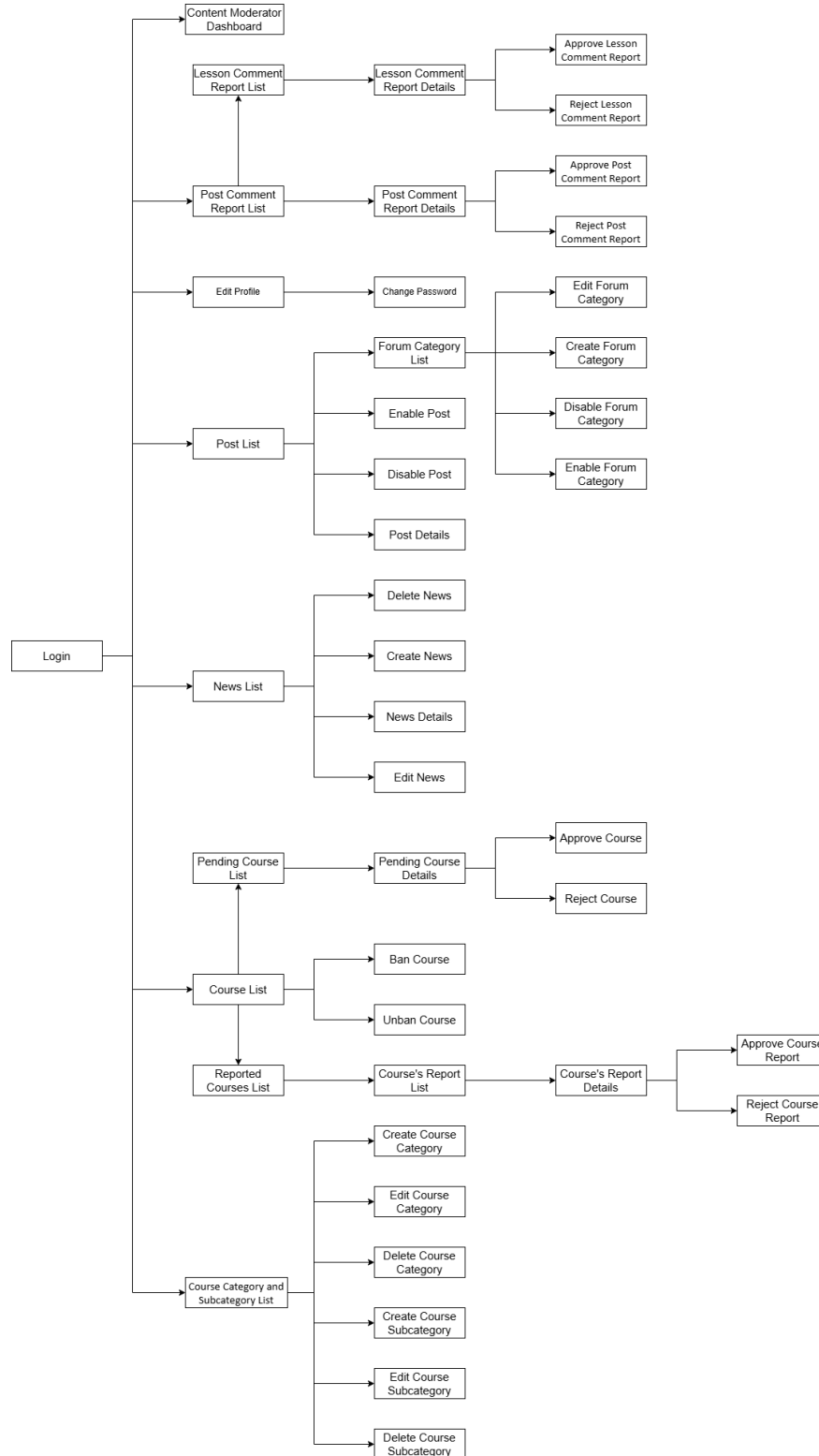
Figure 1.3.1.2 - Content moderator Screens Flow
