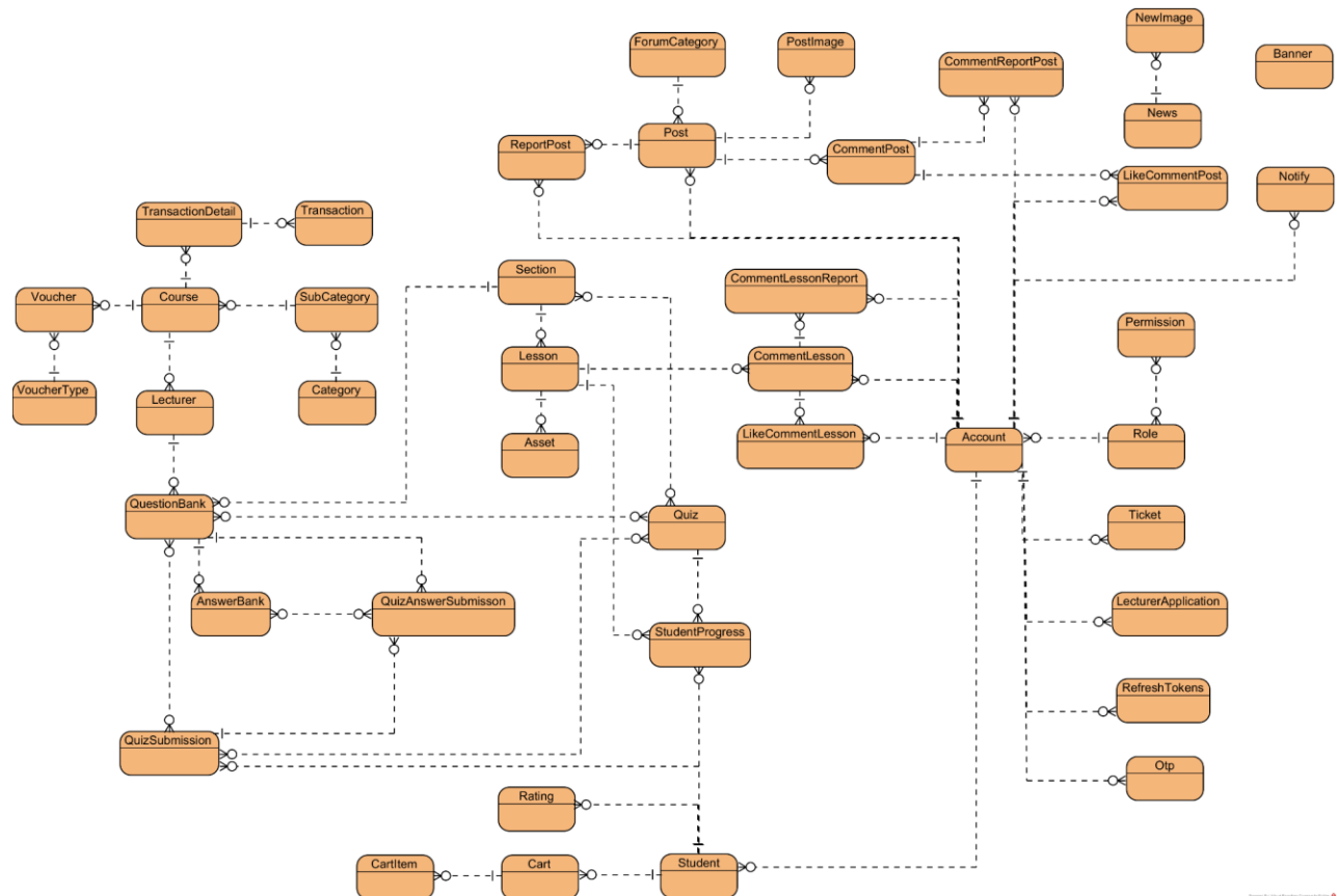
Figure 1.5.1 - Overview entity relationship diagram
