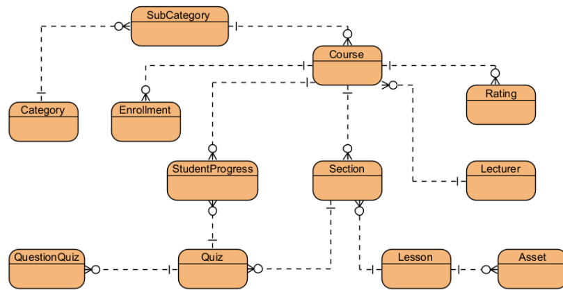
Figure 1.5.3 - Course relationship diagram
