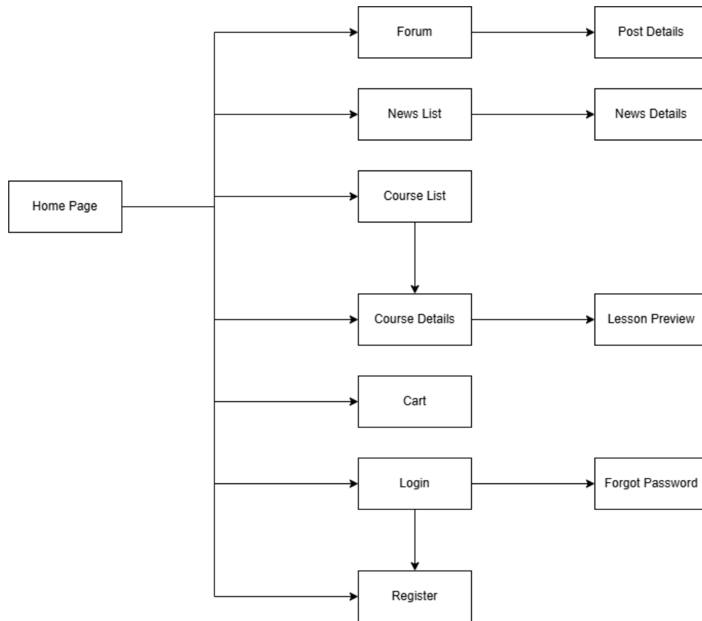
Figure 1.3.1.1 - Guest Screens Flow
