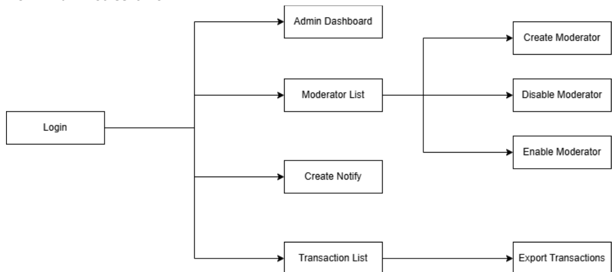
Figure 1.3.1.4 - Admin Screens Flow
