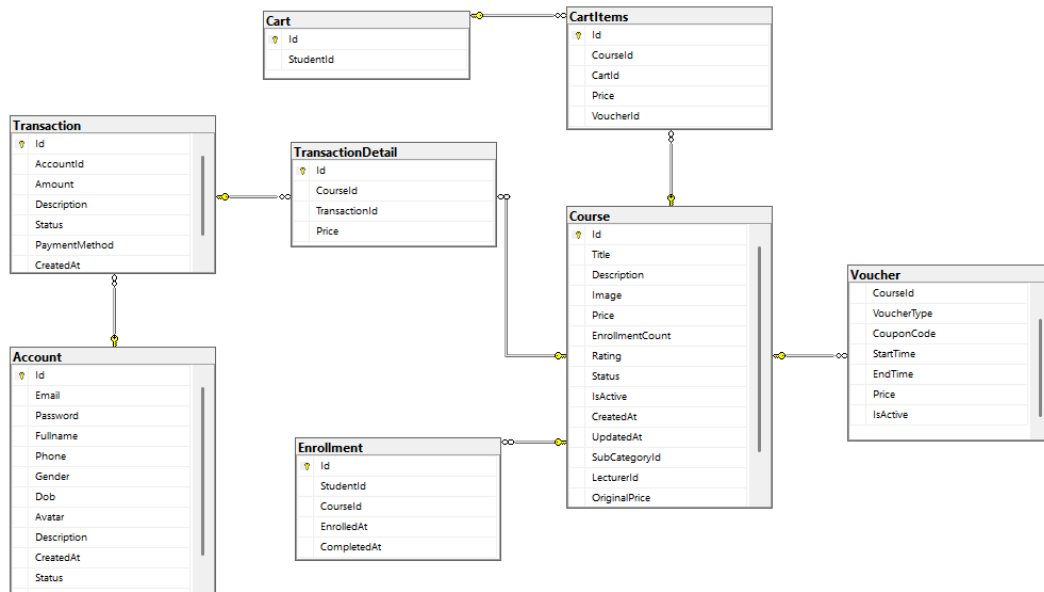
Figure 2.5. - data tables related to shopping cart & payment
