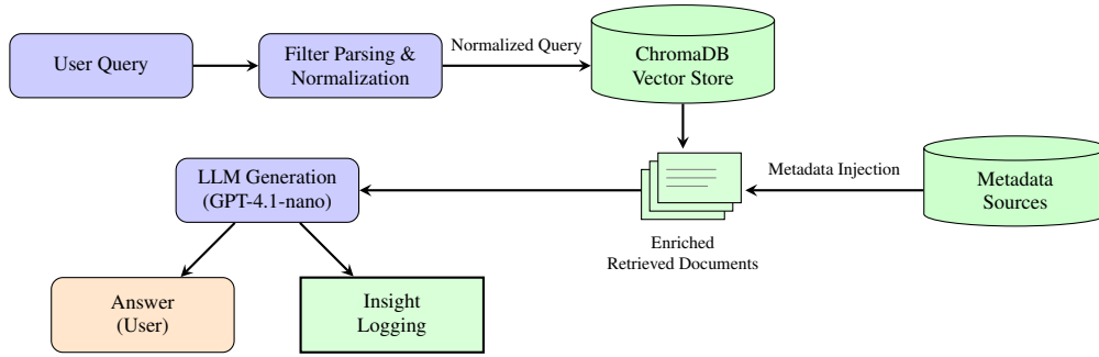
Figure 1: Enhanced RAG system architecture with metadata-guided retrieval, showing the flow from user query through normalized filtering, context enrichment, and answer generation.
