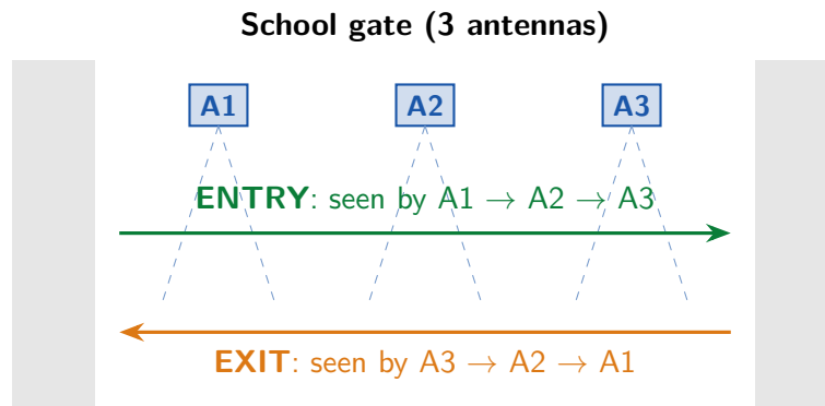
Figure 1.1: The gate has three antennas. The order in which they detect the ID card tells the system whether the student walked in or out.
