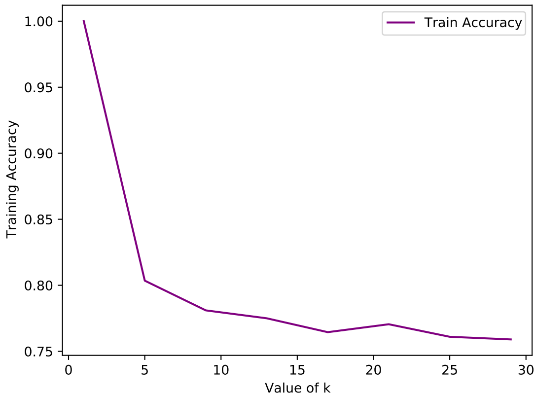
k-NN Performance
