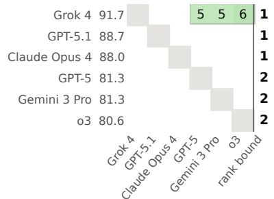
IFEval (541)
