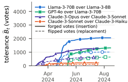
(c) Chatbot Arena, real votes
