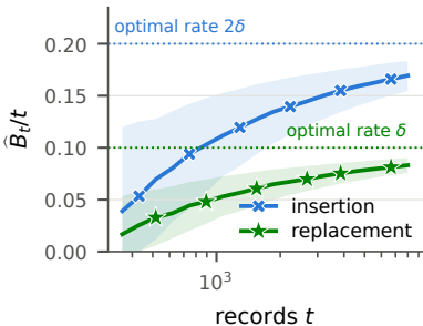
(a) Corruption tolerance per record, \delta = 0.1
