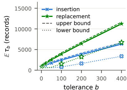
(b) Records to certify, \delta = 0.05
