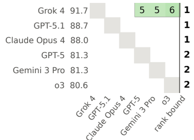
IFEval (541)
