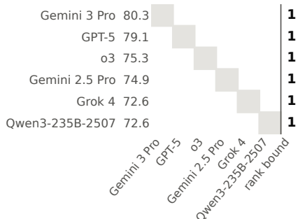
GPQA (446)
