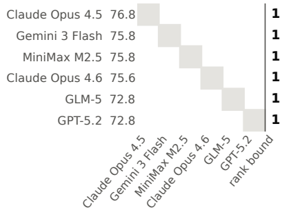
SWE-bench Verified (500)
