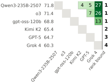
Omni-MATH (1,000)
