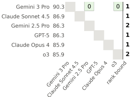
MMLU-Pro (1,000)
