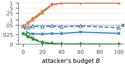
(a) Burst of forged wins
