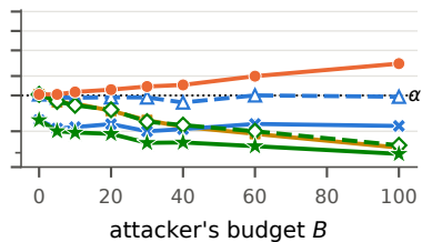
(c) Forged wins at random times
