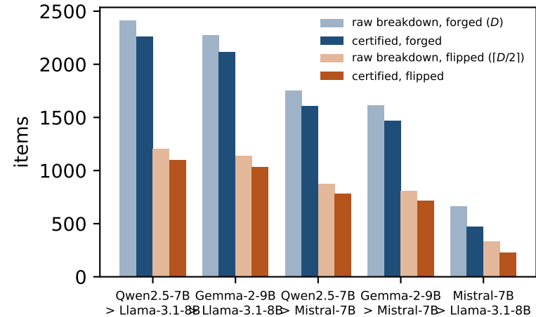
HELM MMLU, 14,042 items: certified budgets
