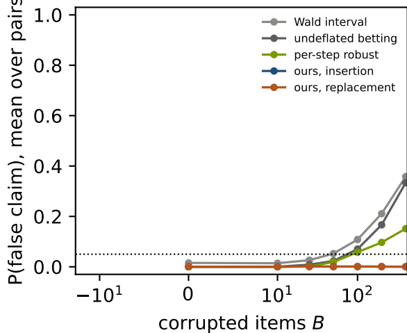
forged items, one burst
