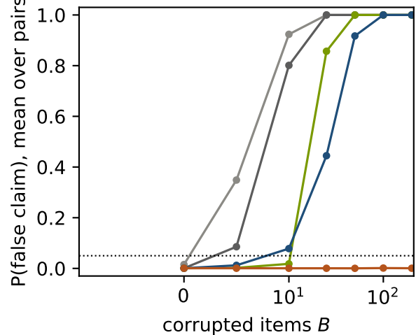
contaminated items (losses flipped)
