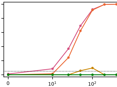
GPQA (446), 103 pairs forged items, one burst
