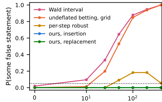
MMLU-Pro (1,000), 103 pairs forged items, one burst
