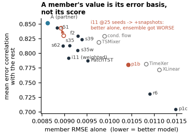
Figure 2: Each object by how good it is alone (horizontal) against how much its errors resemble the rest (vertical). The useful direction is down , not left. The three stock-flow models are the worst in the set and the only ones far from the crowd. The arrow shows a member being genuinely improved: it moves left and also up, and the ensemble got worse.
