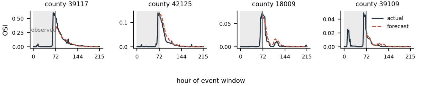
Figure 4: Forecasts for four counties never seen in training, spanning the severity range. Shaded: the 72 observed hours. Everything after is predicted.
