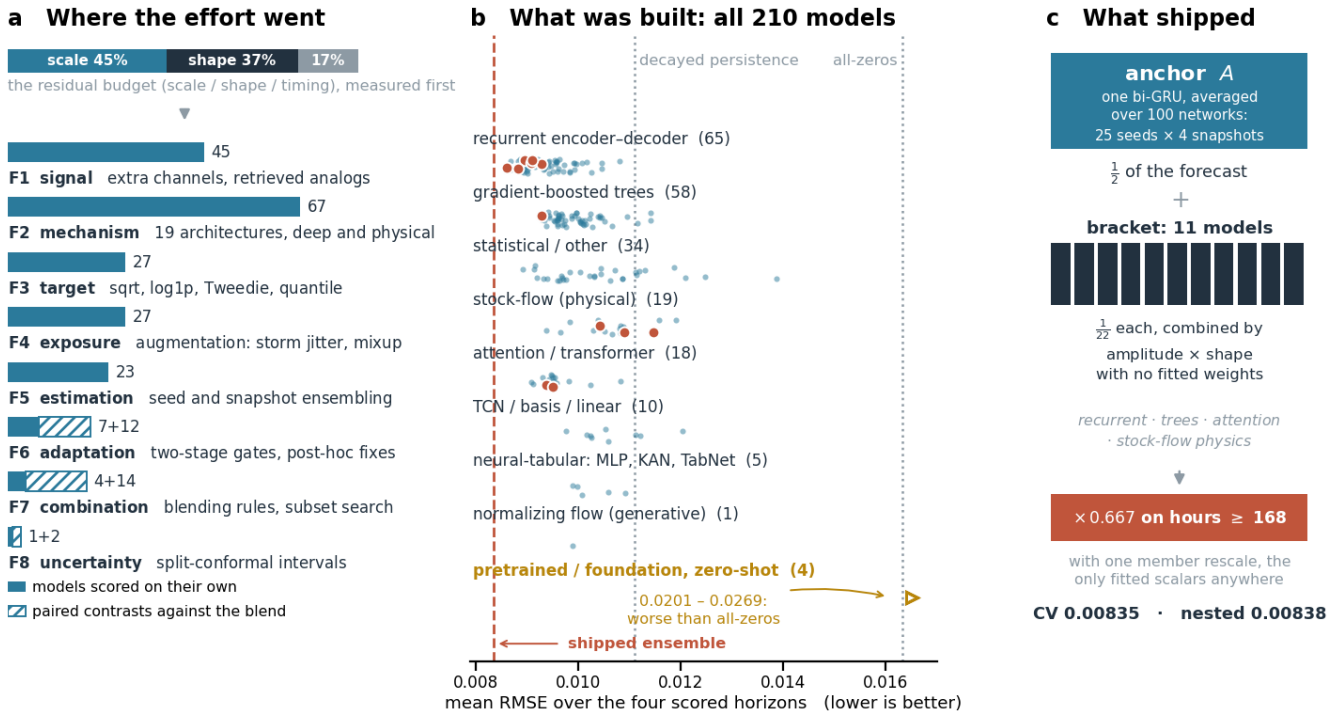
Figure 2: The whole procedure. (a) A residual budget measured before any model existed allocated attention across eight families; solid bars are models scored on their own, hatched bars are paired contrasts against the blend. (b) All 210 models, by class and by score under the single protocol of Table 1; the twelve that shipped are ringed. Only the four pretrained forecasters fall off the axis — they lose to predicting zero everywhere. (c) What survived: one heavily averaged anchor holding half the forecast, eleven dissimilar models sharing the other half, one quiet-tail scalar, and no fitted combination weight anywhere.
