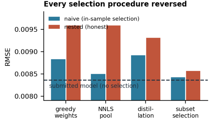
Figure 1: Left: squared error against counties ranked by their contribution — 14 counties carry 65%. Right: four selection procedures, scored naively and with the selection itself nested inside the folds. Every one reverses.
