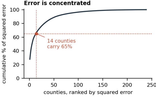
Figure 1: Left: squared error against counties ranked by their contribution — 14 counties carry 65%. Right: four selection procedures, scored naively and with the selection itself nested inside the folds. Every one reverses.
