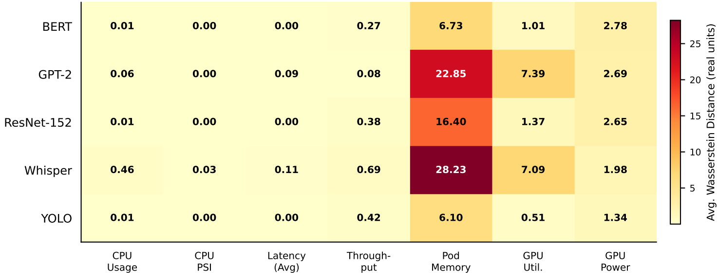
Wasserstein Distance: Real vs. Synthetic (S36) Averaged over r = 1\text{--}10 , lower is better
