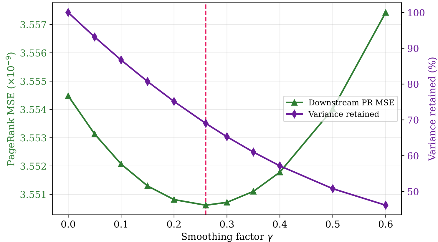
Downstream Stability: PageRank MSE and Signal Variance vs. Smoothing Factor \gamma (49 CV splits)
