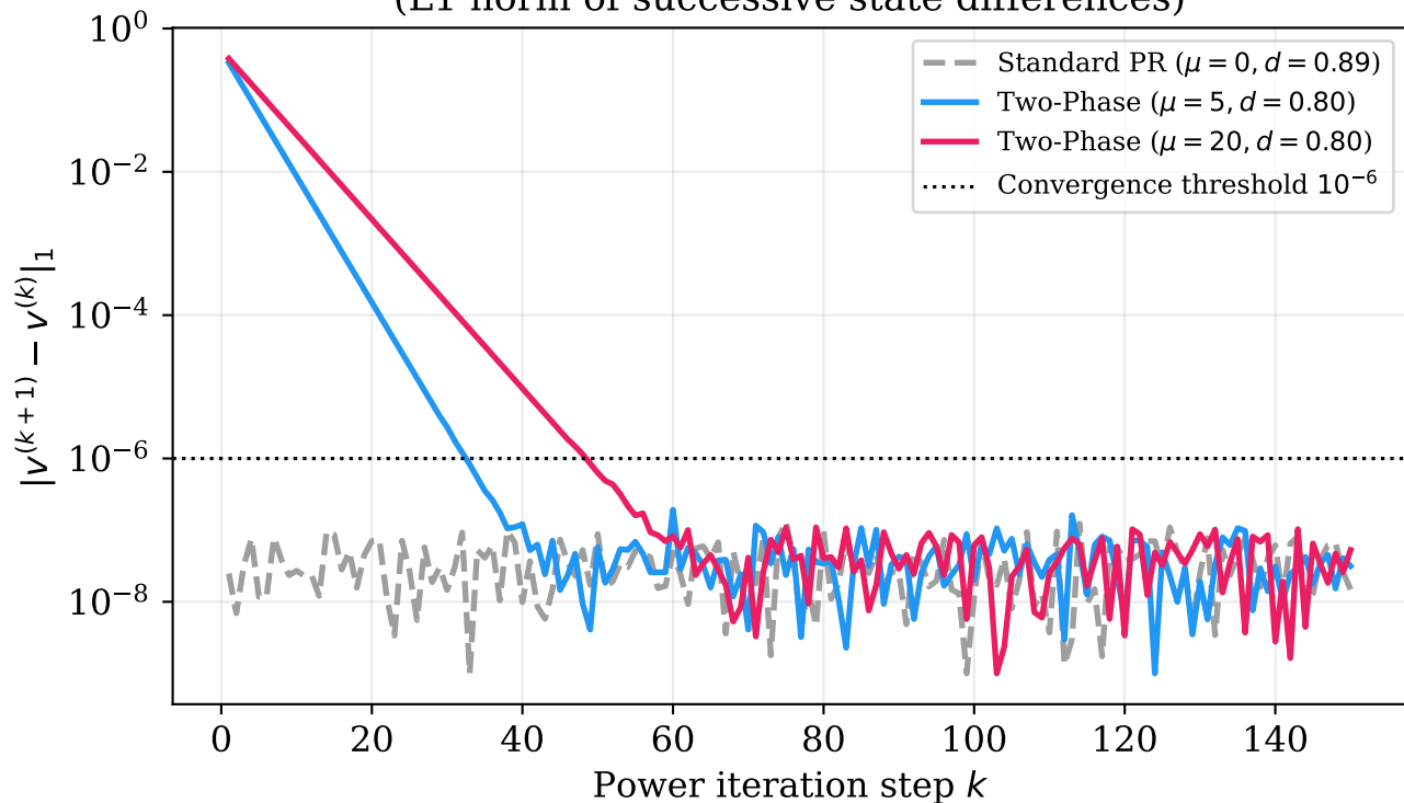
Convergence of Power Iteration (L1 norm of successive state differences)
