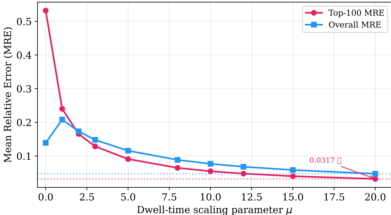
Effect of \mu on Prediction Accuracy ( d = 0.80 , \beta = 0.90 )
