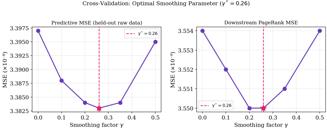
Figure 6: Predictive MSE and downstream PageRank MSE side by side, both minimised at \gamma^* = 0.26 .
