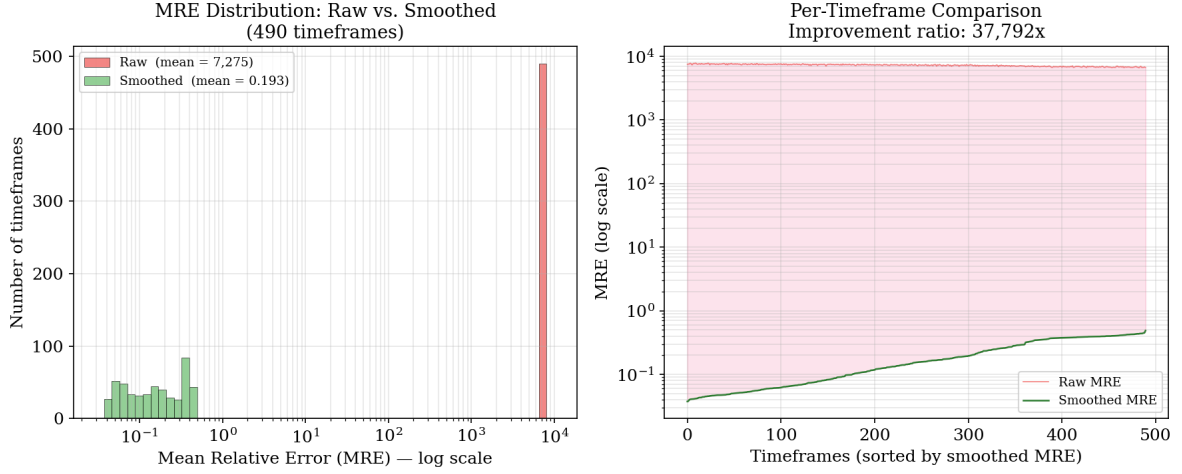
Figure 7: Per-timeframe MRE comparison across 490 windows. Left: log-scale histogram showing the raw pipeline clustered around MRE \approx 7,000 while the smoothed pipeline achieves MRE \approx 0.19 . Right: sorted per-timeframe comparison showing a consistent \sim 4 orders-of-magnitude gap.
