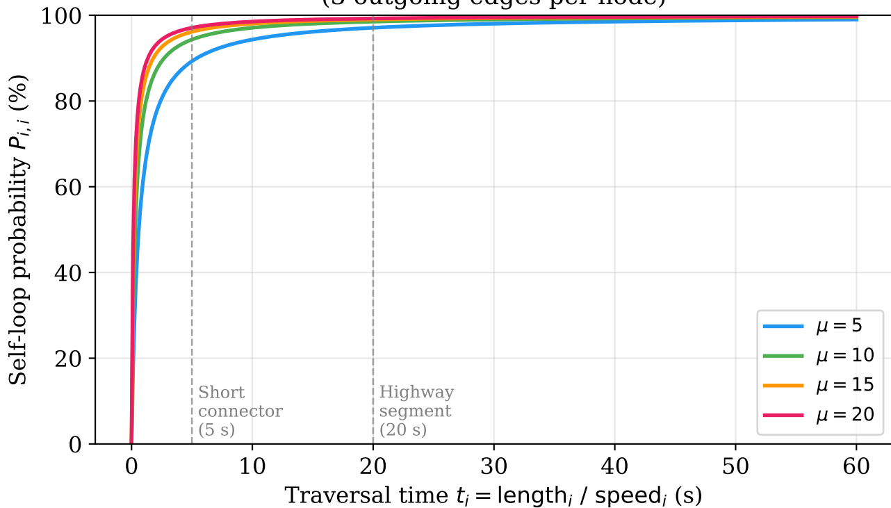
Self-Loop Probability vs. Traversal Time (3 outgoing edges per node)
