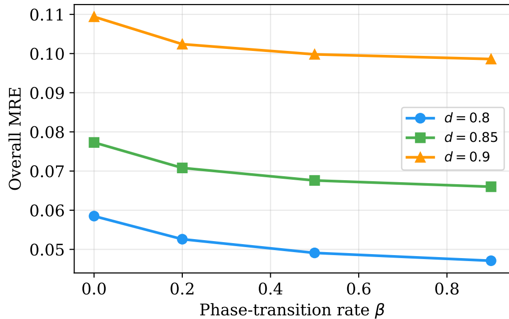
Overall MRE vs. \beta and d ( \mu = 20 )
