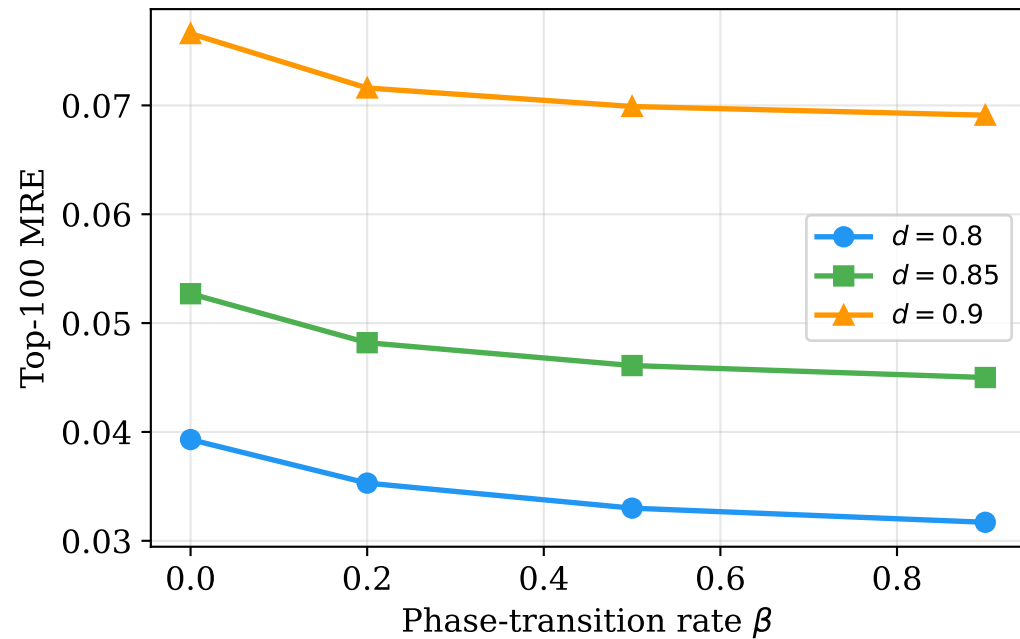
Top-100 MRE vs. \beta and d ( \mu = 20 )
