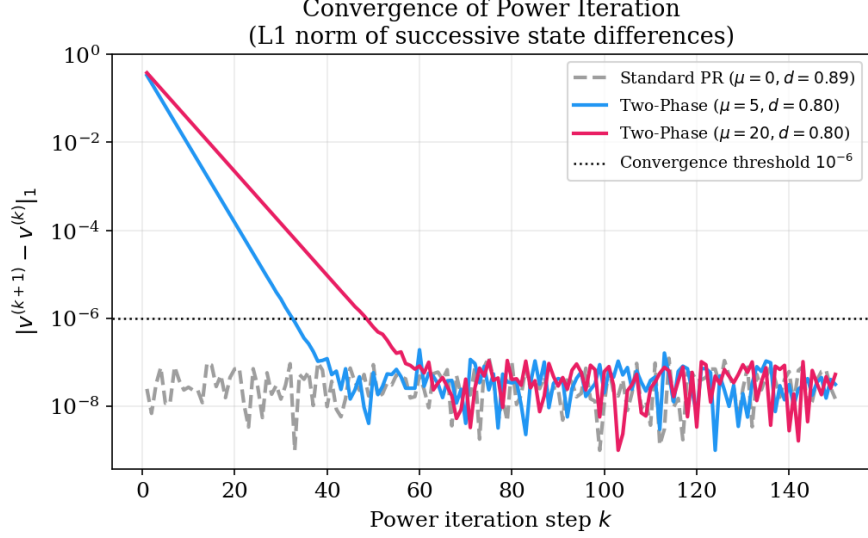
Figure 12: Simulated convergence curves (L1 norm of consecutive differences). Higher \mu increases the effective spectral gap, leading to faster convergence compared to standard PageRank.
