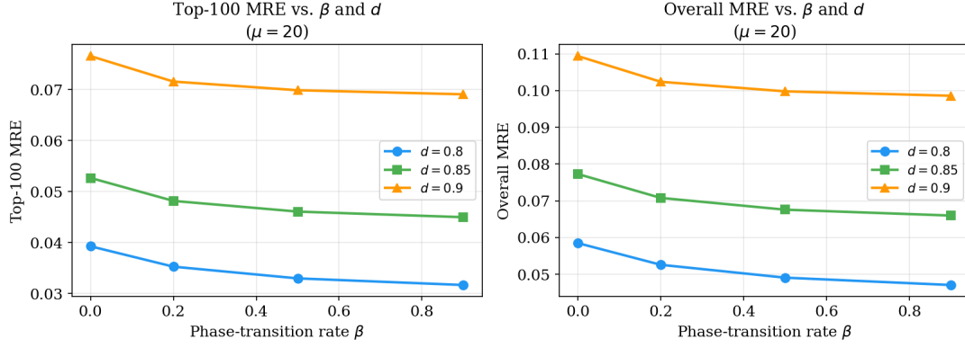
Figure 15: Sensitivity of Top-100 and Overall MRE to the damping factor d and phase-transition rate \beta , with \mu = 20 fixed.
