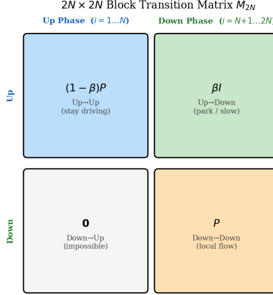
Figure 10: Visual structure of the 2N \times 2N block transition matrix. The bottom-left block is identically zero, enforcing the one-way phase transition.
