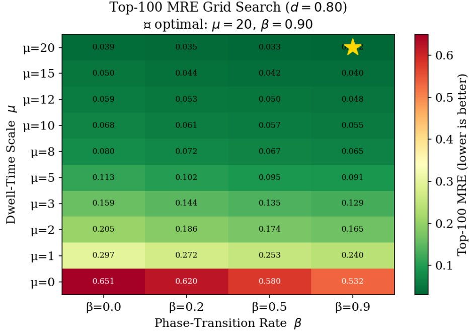
Figure 14: Heatmap of Top-100 MRE for d = 0.80 over all tested (\mu, \beta) pairs. The star marks the global optimum at \mu = 20, \beta = 0.90 .
