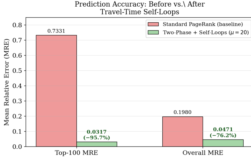
Figure 16: Bar chart comparing baseline (standard PageRank) against the optimised Two-Phase + Self-Loop model. The 95.7% Top-100 improvement is simultaneous with a 76.2% overall improvement.
